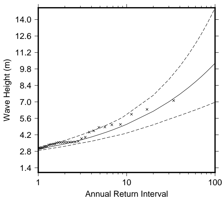
Figure 9 Extreme wave distribution for Mango Bay_Resort. The crosses represents the wave events that occurred since 1979. The plain line is the statistical distribution that best fit the past wave events. The dotted line show the upper and lower high confidence of the fit, there is a 95% chance that the fitted distribution lie between the two dashed lines.
