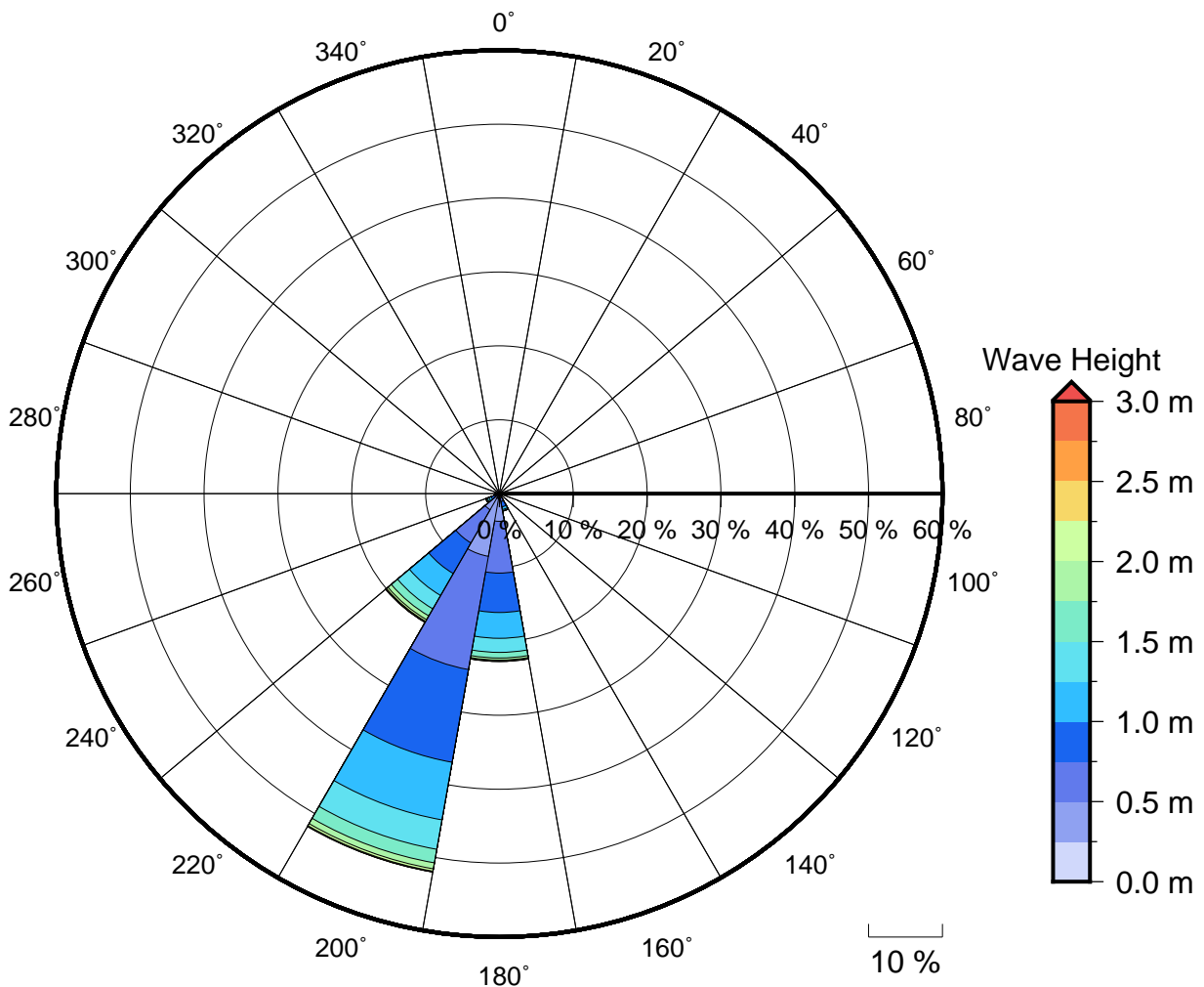
Figure 2 Annual wave rose for Mango Bay_Resort. Note that direction are where the wave are coming from.
