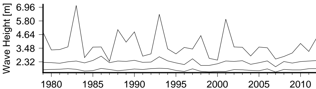
Figure 8 Annual variation in large waves (90th percentile)(lower curve), severe waves (99th percentile) (middle curve) and the largest wave(upper curve) in Mango Bay_Resort.
