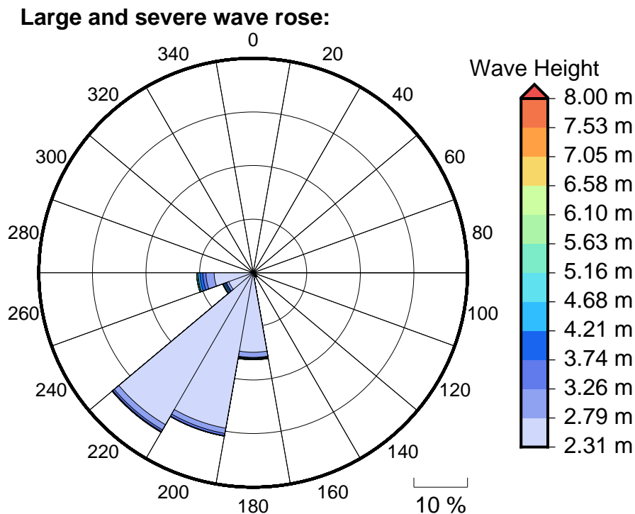
Figure 6 Large, severe and extreme wave roses for Mango Bay_Resort
