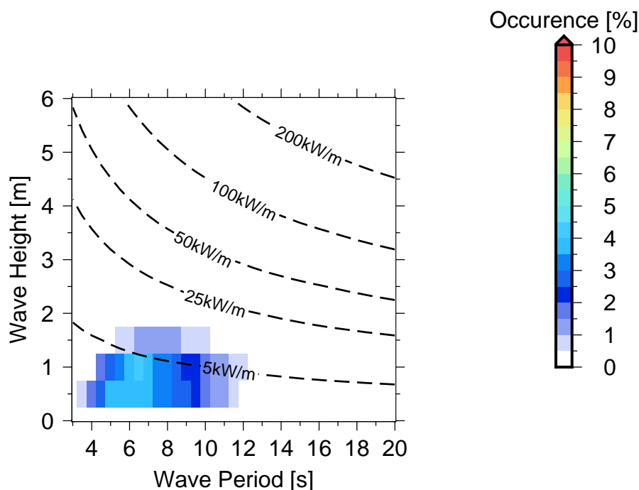
Figure 10 Occurrences of sea states in Mango Bay_Resort .
