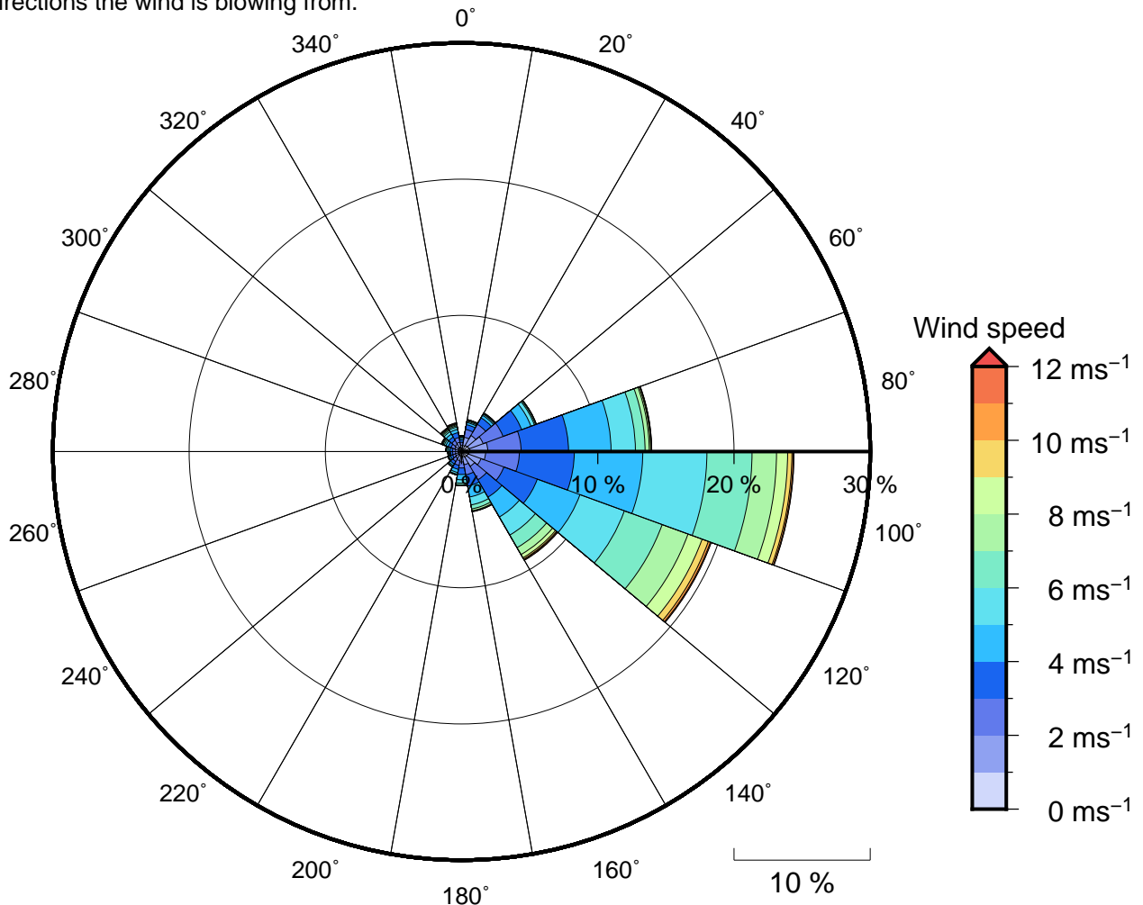
Figure 11 Annual wind rose for Mango Bay_Resort. Note that directions are where the wind is coming from.
