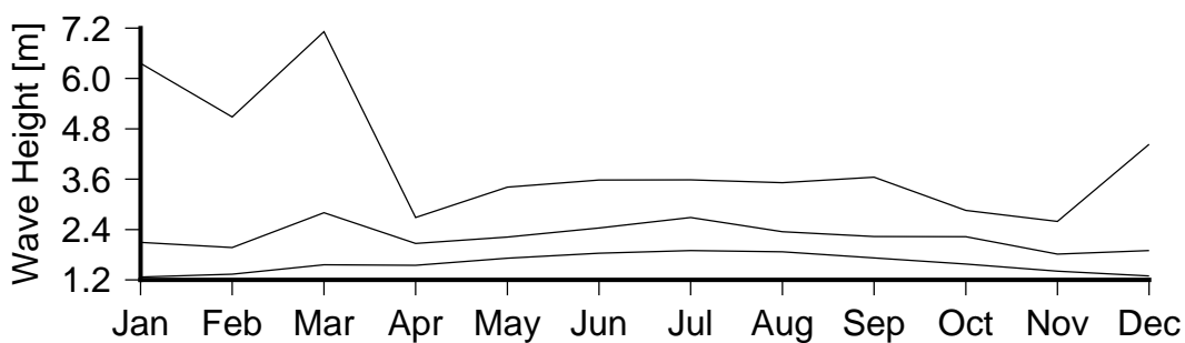
Figure 7 Monthly variation in large waves (90th percentile)(lower curve), severe waves (99th percentile) (middle curve) and the largest wave(upper curve) in Mango Bay_Resort.
