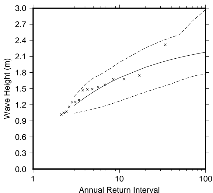
Figure 9 Extreme wave distribution for Malolo Marina. The crosses represents the wave events that occurred since 1979. The plain line is the statistical distribution that best fit the past wave events. The dotted line show the upper and lower high confidence of the fit, there is a 95% chance that the fitted distribution lie between the two dashed lines.
