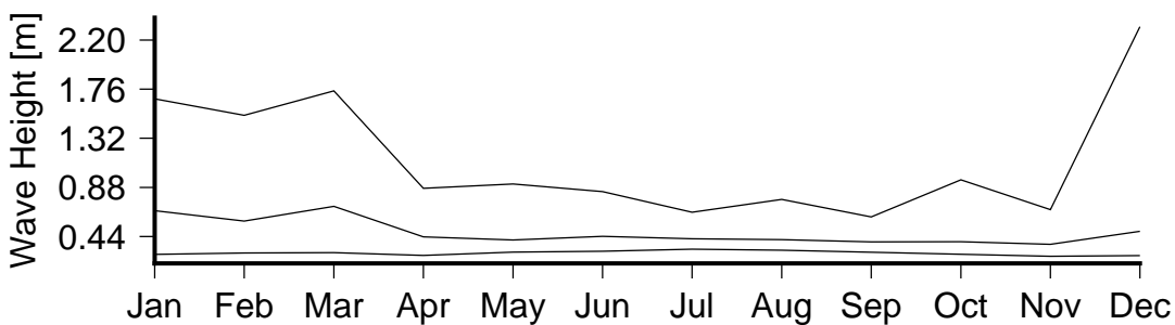
Figure 7 Monthly variation in large waves (90th percentile)(lower curve), severe waves (99th percentile) (middle curve) and the largest wave(upper curve) in Malolo Marina.
