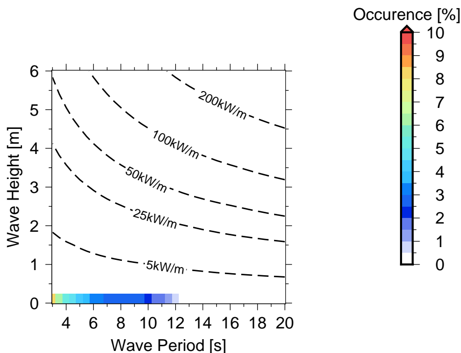
Figure 10 Occurences of sea states in Malolo Marina .
