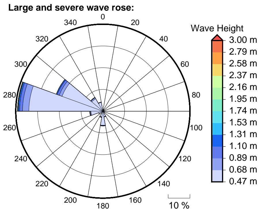
Figure 6 Large, severe and extreme wave roses for Malolo Marina
