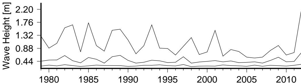
Figure 8 Annual variation in large waves (90th percentile)(lower curve), severe waves (99th percentile) (middle curve) and the largest wave(upper curve) in Malolo Marina.
