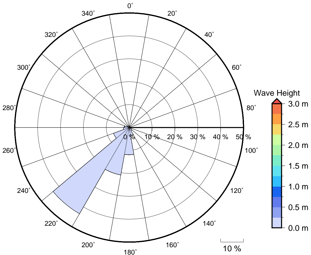
Figure 2 Annual wave rose for Malolo Marina. Note that direction are where the wave are coming from .
