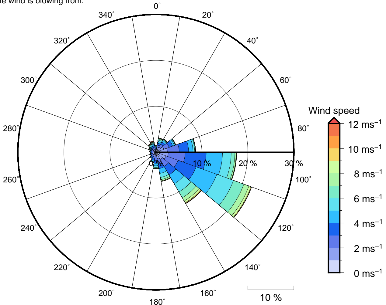
Figure 11 Annual wind rose for Malolo Marina. Note that directions are where the wind is coming from.
