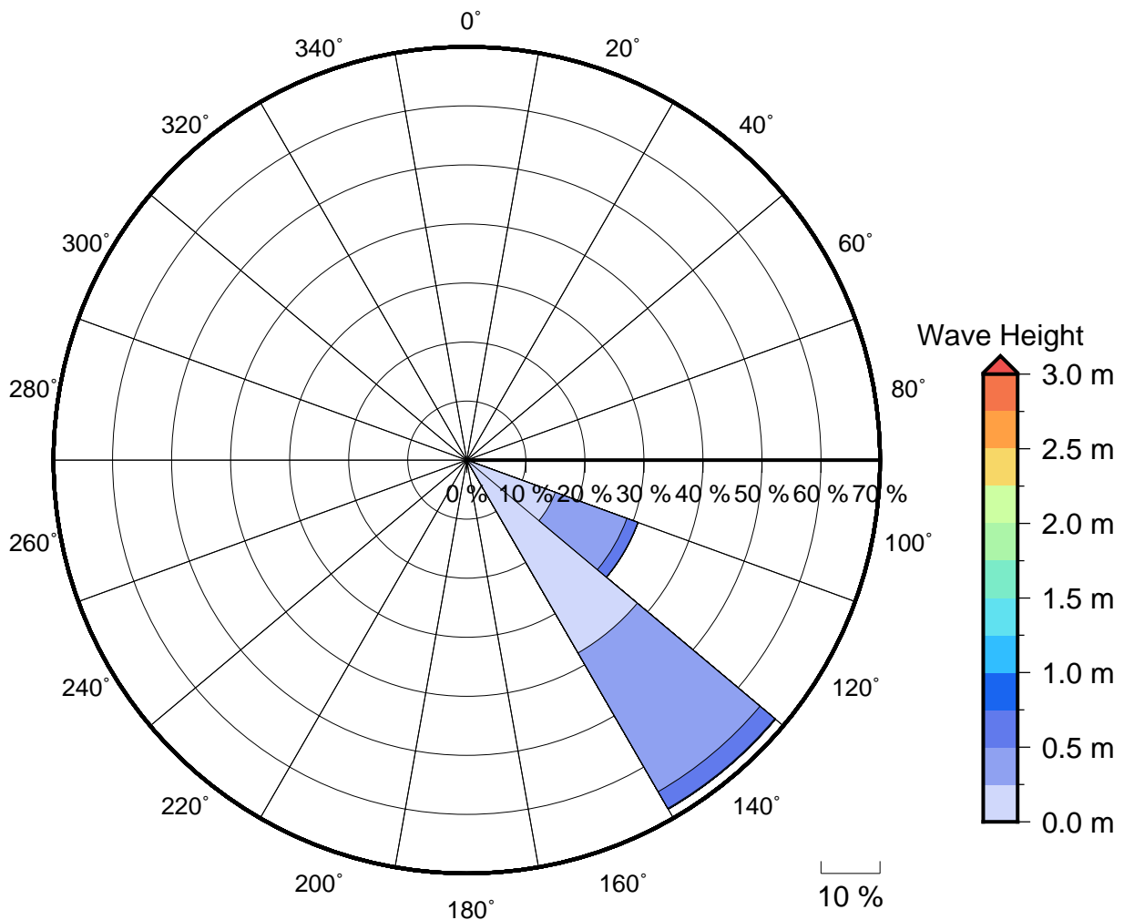
Figure 2 Annual wave rose for Laucala Bay. Note that direction are where the wave are coming from .
