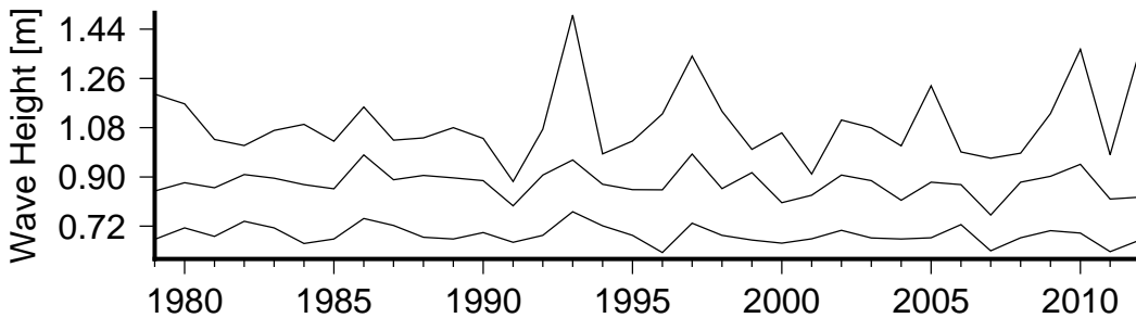
Figure 8 Annual variation in large waves (90th percentile)(lower curve), severe waves (99th percentile) (middle curve) and the largest wave(upper curve) in Laucala Bay.
