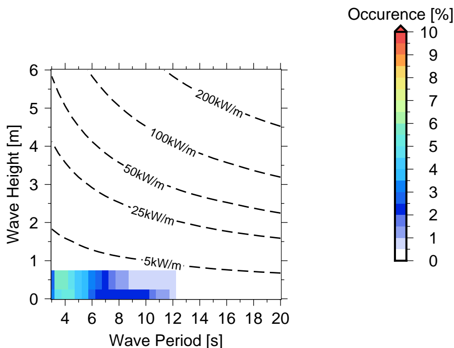
Figure 10 Occurrences of sea states in Laucala Bay .
