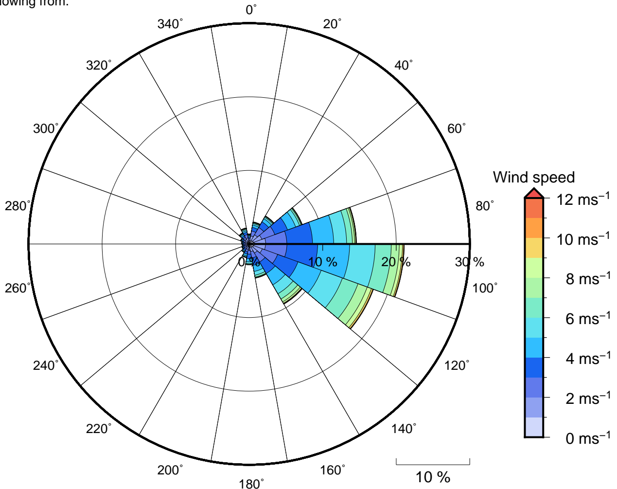
Figure 11 Annual wind rose for Laucala Bay. Note that directions are where the wind is coming from
