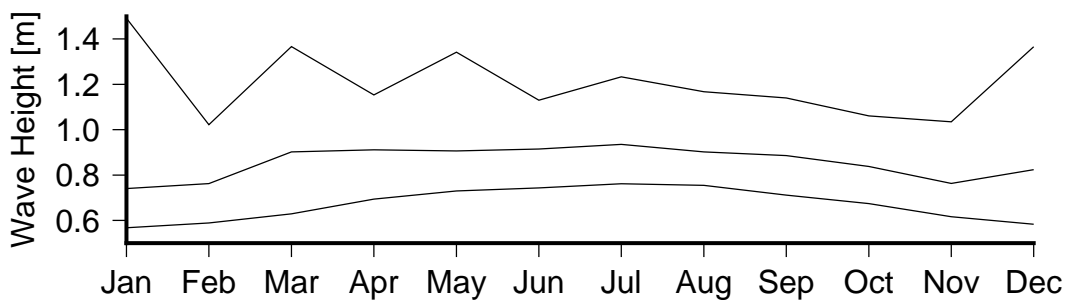
Figure 7 Monthly variation in large waves (90th percentile)(lower curve), severe waves (99th percentile) (middle curve) and the largest wave(upper curve) in Laucala Bay.
