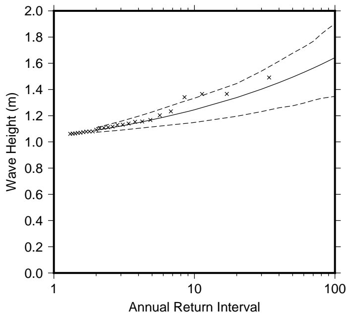
Figure 9 Extreme wave distribution for Laucala Bay. The crosses represents the wave events that occurred since 1979. The plain line is the statistical distribution that best fit the past wave events. The dotted line show the upper and lower high confidence of the fit, there is a 95% chance that the fitted distribution lie between the two dashed lines.
