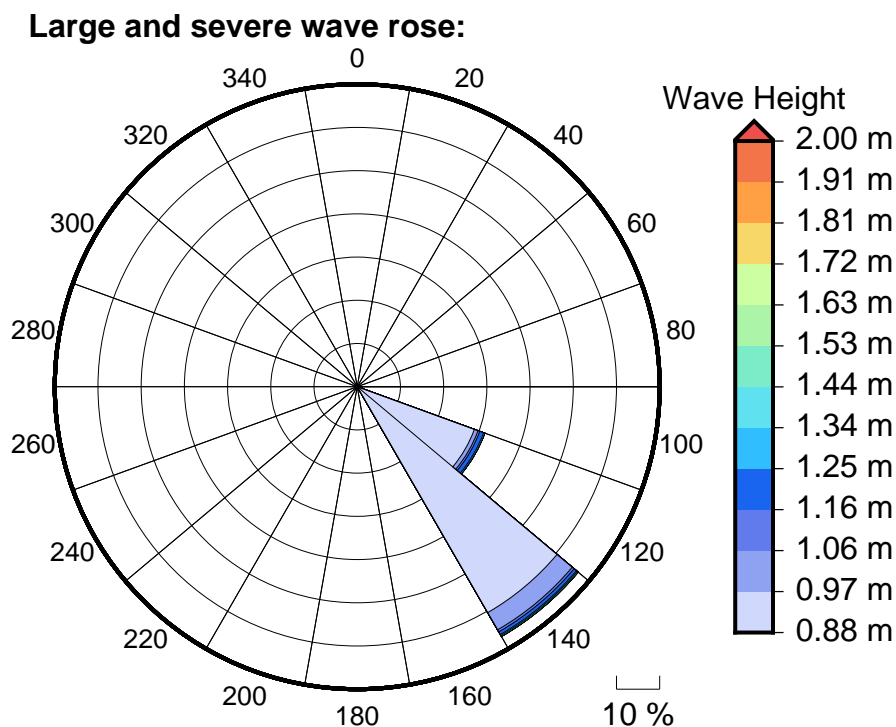
Figure 6 Large, severe and extreme wave roses for Laucala Bay
