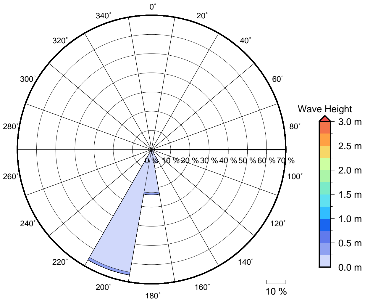
Figure 2 Annual wave rose for Lami. Note that direction are where the wave are coming from.
