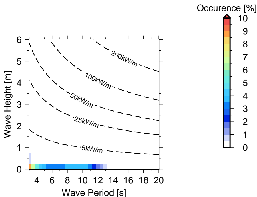
Figure 10 Occurrences of sea states in Lami .
