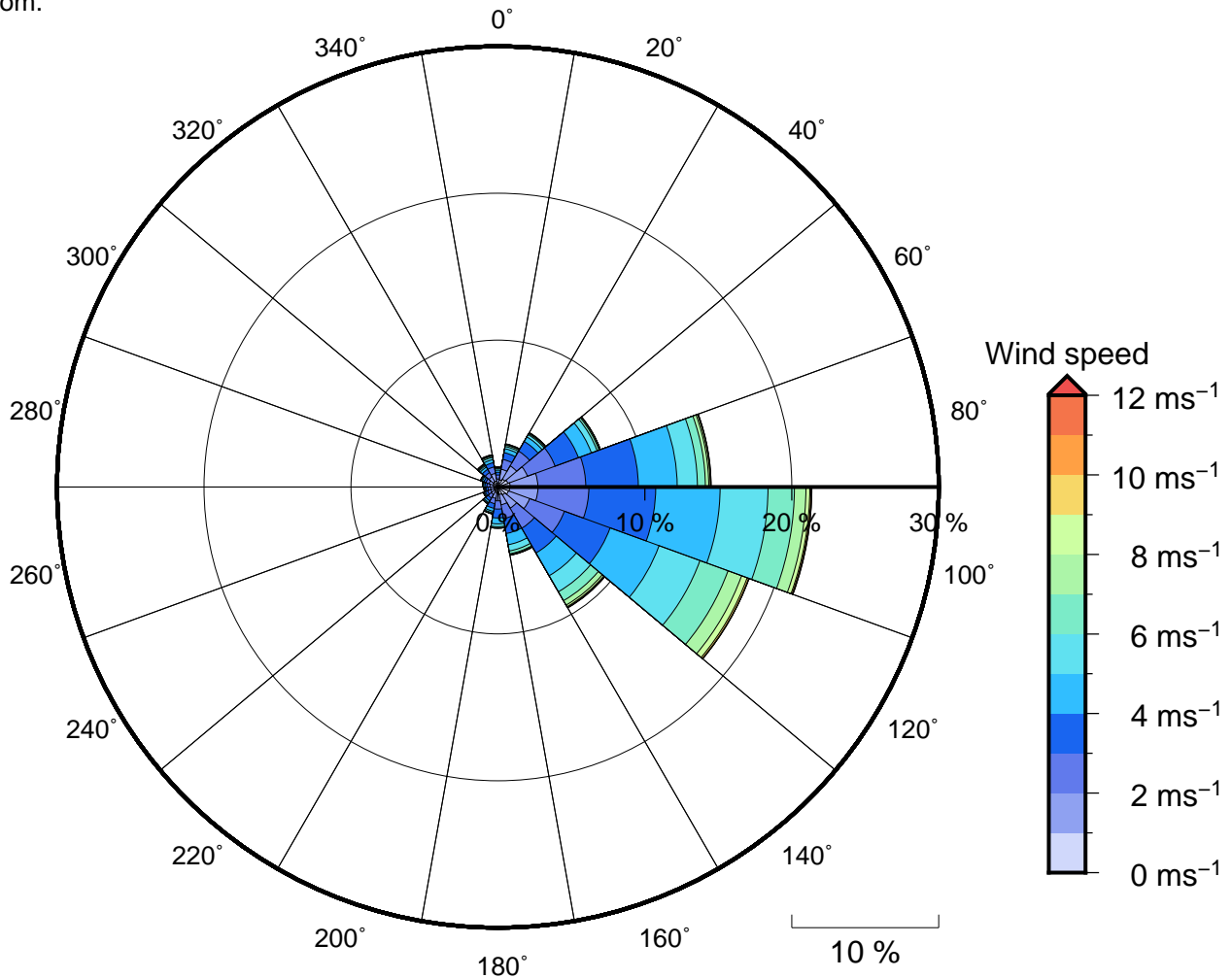
Figure 11 Annual wind rose for Lami. Note that directions are where the wind is coming from.
