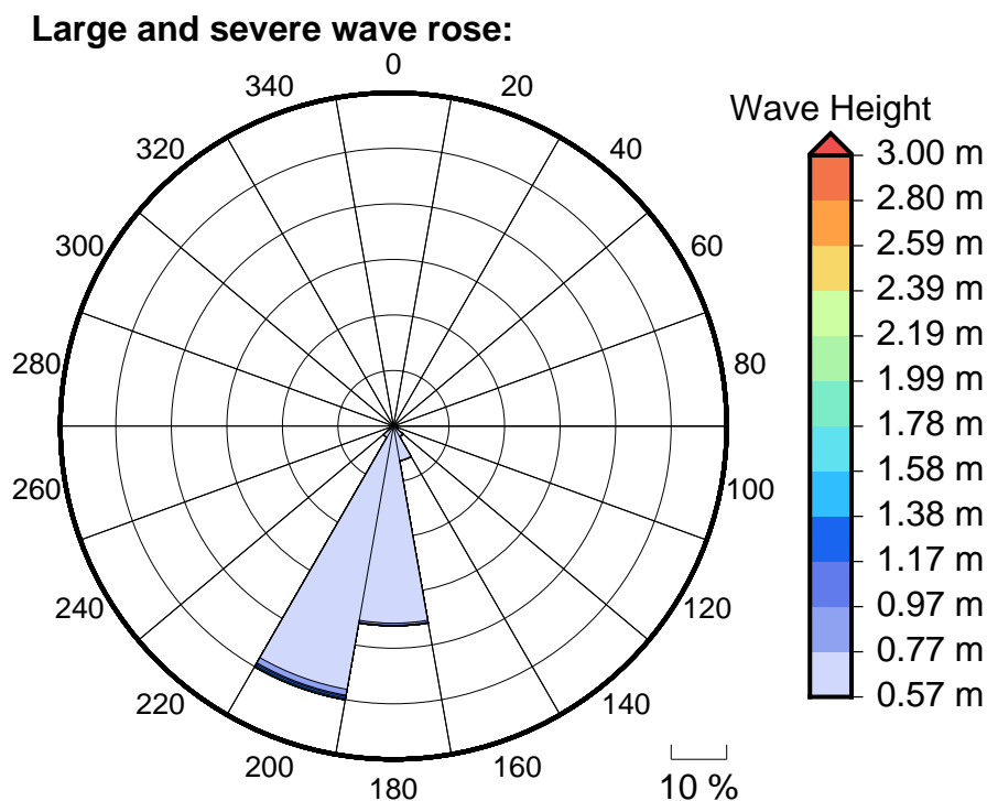
Figure 6 Large, severe and extreme wave roses for Lami
