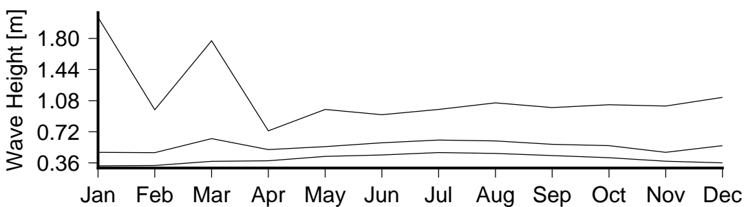
Figure 7 Monthly variation in large waves (90th percentile)(lower curve), severe waves (99th percentile) (middle curve) and the largest wave(upper curve) in Lami.
