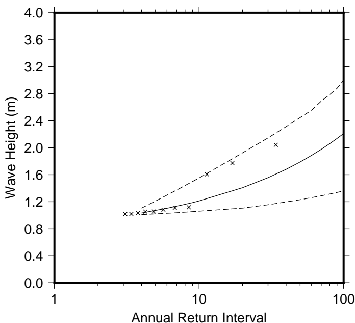
Figure 9 Extreme wave distribution for Lami. The crosses represents the wave events that occurred since 1979. The plain line is the statistical distribution that best fit the past wave events. The dotted line show the upper and lower high confidence of the fit, there is a 95% chance that the fitted distribution lie between the two dashed lines.
