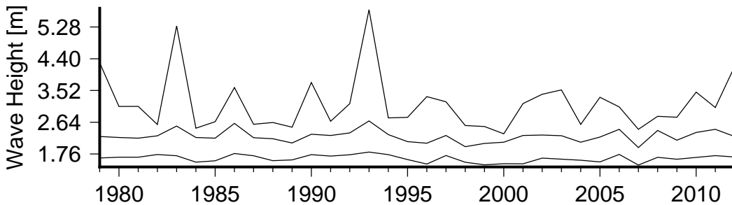
Figure 8 Annual variation in large waves (90th percentile)(lower curve), severe waves (99th percentile) (middle curve) and the largest wave(upper curve) in Korolevu Bay.
