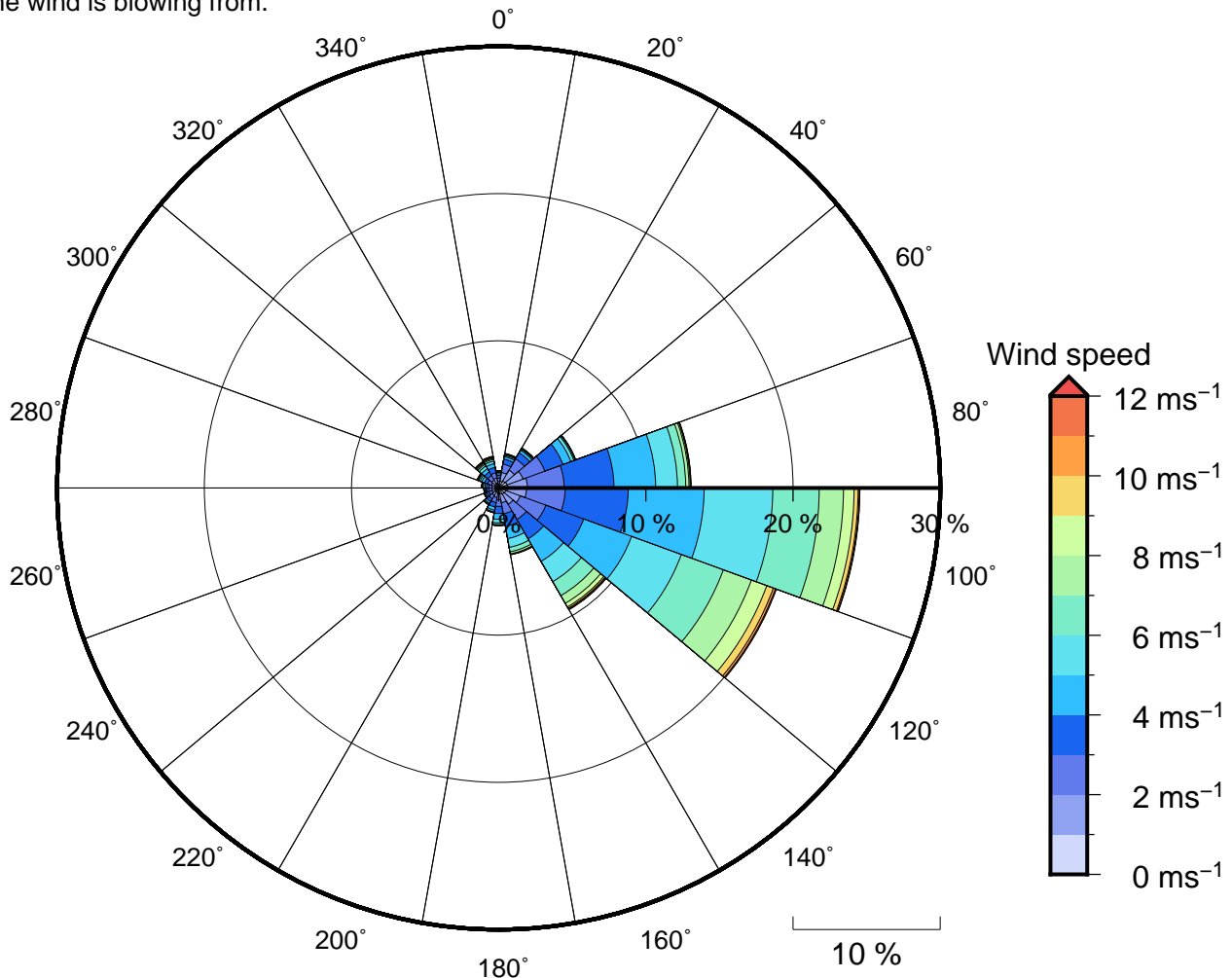
Figure 11 Annual wind rose for Korolevu Bay. Note that directions are where the wind is coming from.
