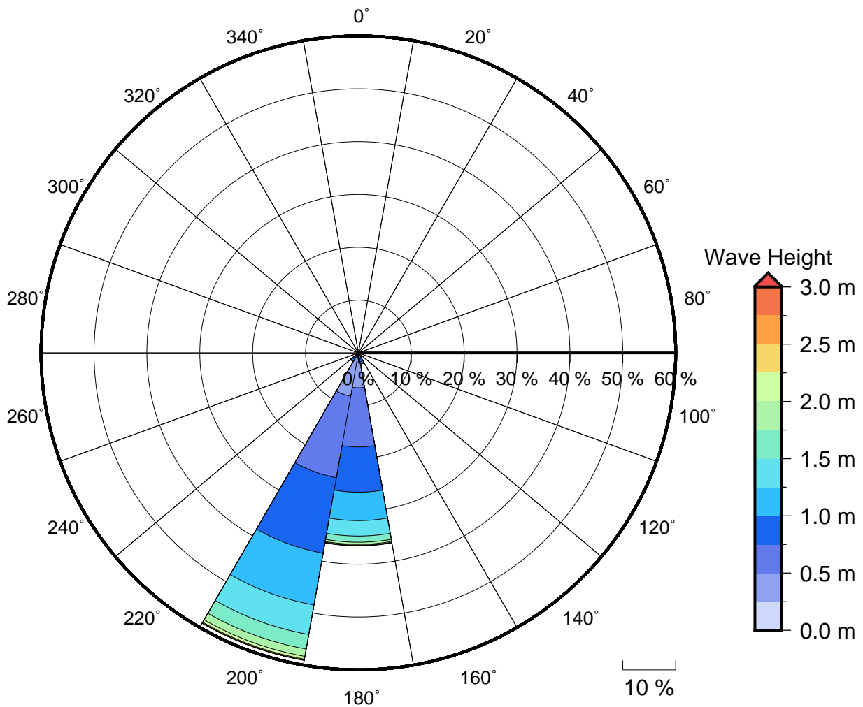
Figure 2 Annual wave rose for Korolevu Bay. Note that direction are where the wave are coming from .
