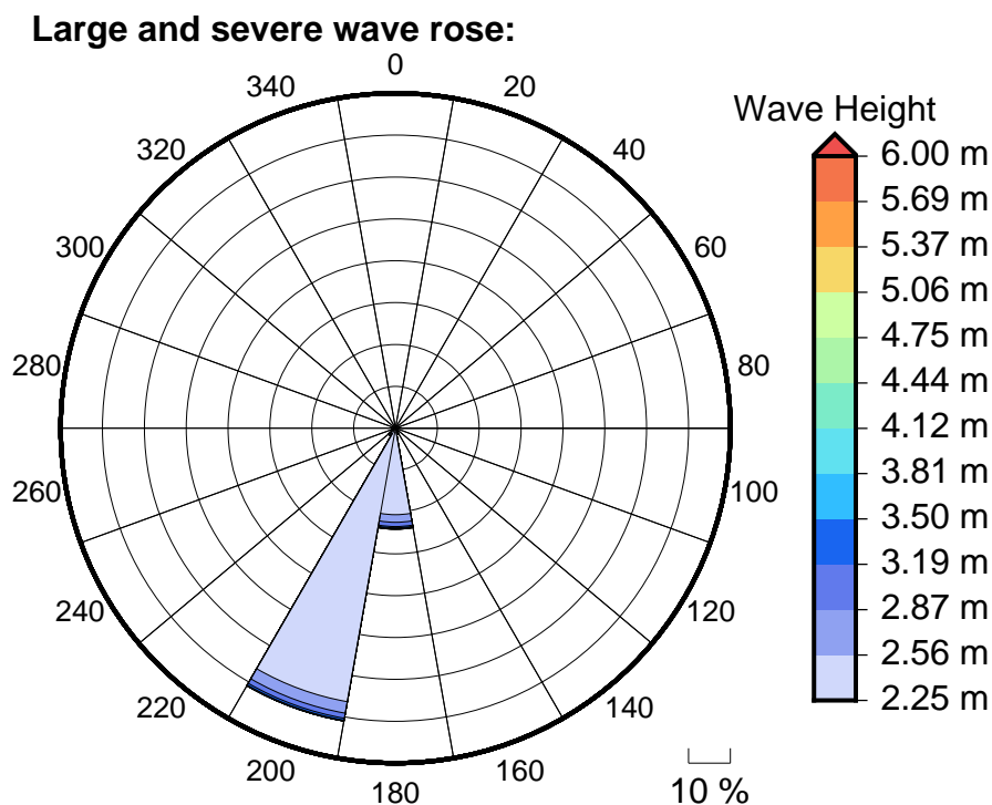
Figure 6 Large, severe and extreme wave roses for Korolevu Bay
