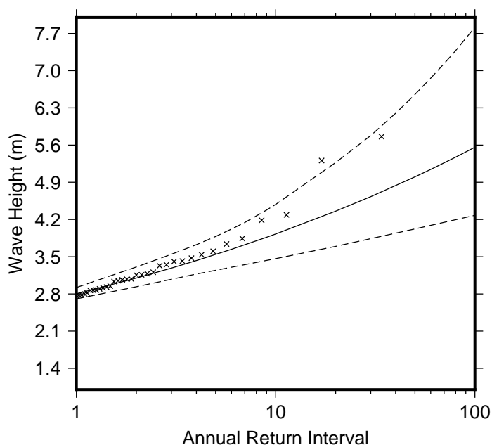
Figure 9 Extreme wave distribution for Korolevu Bay. The crosses represents the wave events that occurred since 1979. The plain line is the statistical distribution that best fit the past wave events. The dotted line show the upper and lower high confidence of the fit, there is a 95% chance that the fitted distribution lie between the two dashed lines.
