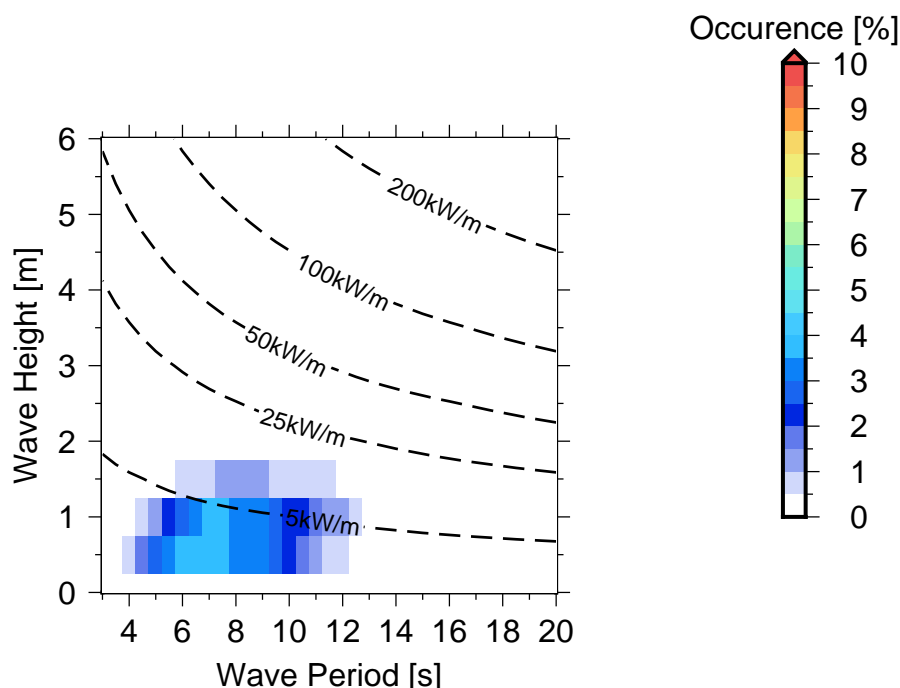
Figure 10 Occurrences of sea states in Korolevu Bay .
