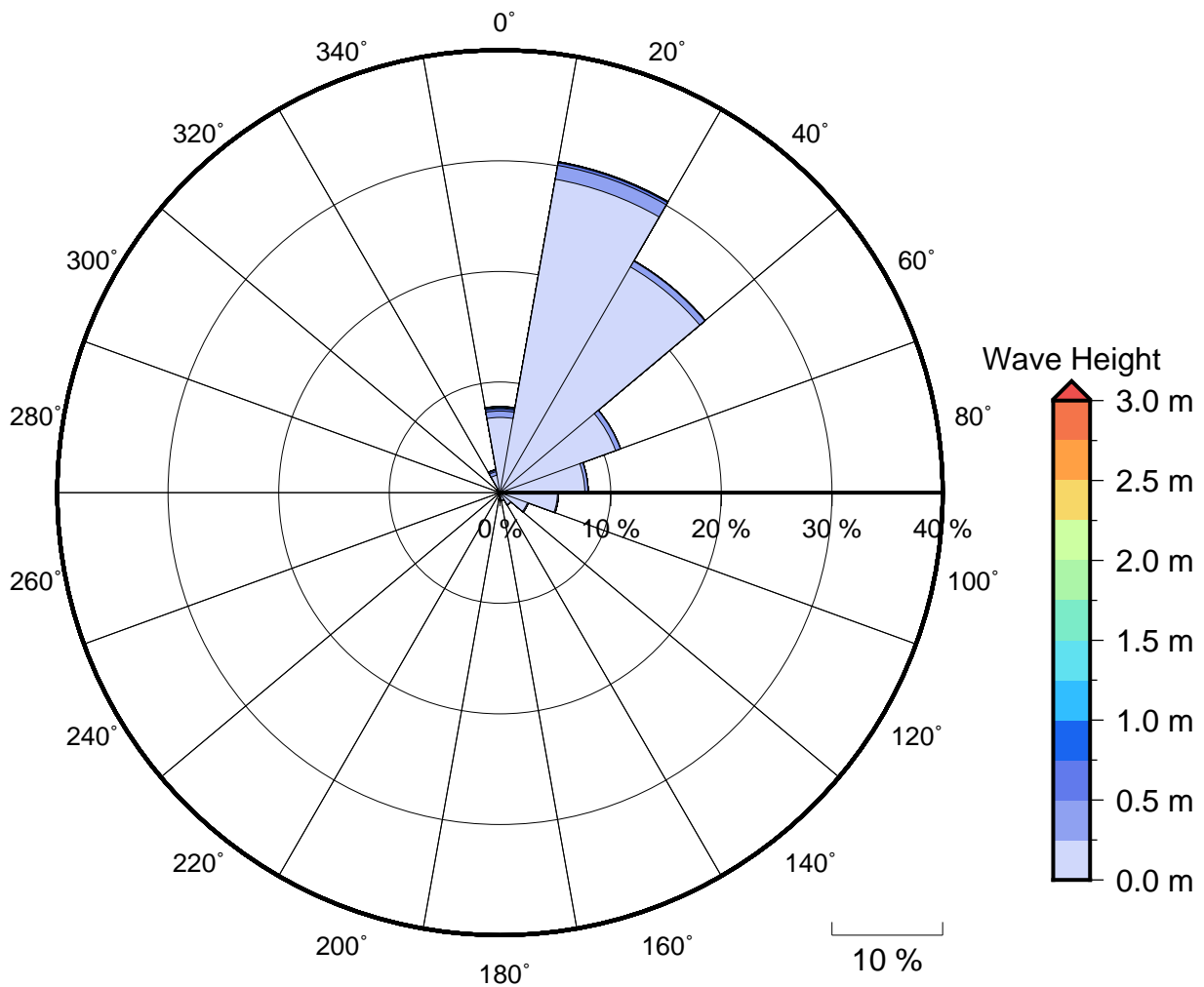
Figure 2 Annual wave rose for Kavala Bay. Note that direction are where the wave are coming from.
