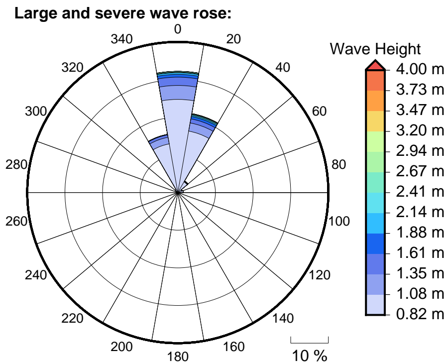
Figure 6 Large, severe and extreme wave roses for Kavala Bay
