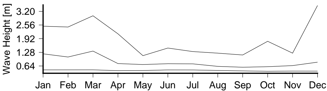
Figure 7 Monthly variation in large waves (90th percentile)(lower curve), severe waves (99th percentile) (middle curve) and the largest wave(upper curve) in Kavala Bay.
