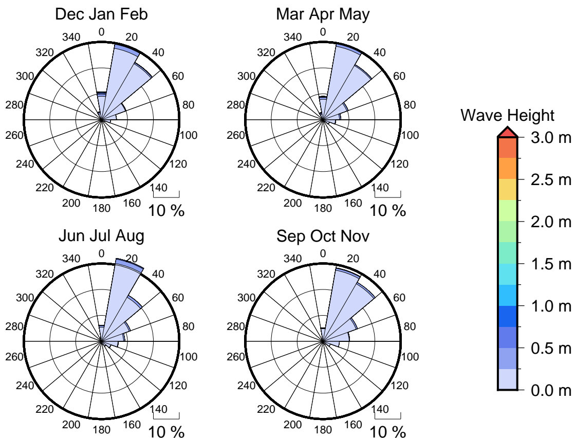
Figure 3 Seasonal wave roses for Kavala Bay
