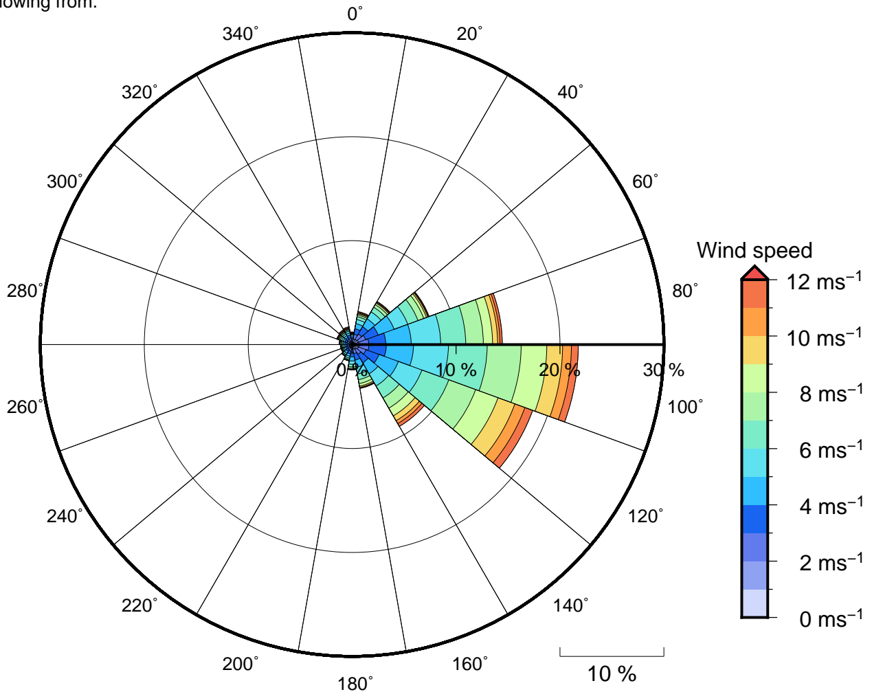
Figure 11 Annual wind rose for Kavala Bay. Note that directions are where the wind is coming from .
