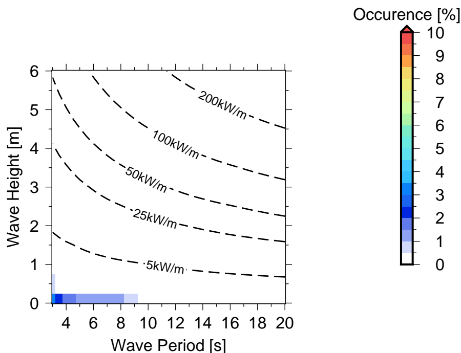
Figure 10 Occurrences of sea states in Kavala Bay .
