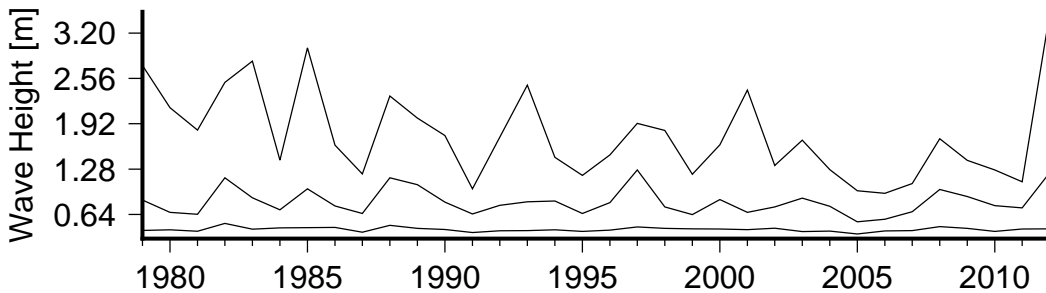
Figure 8 Annual variation in large waves (90th percentile)(lower curve), severe waves (99th percentile) (middle curve) and the largest wave(upper curve) in Kavala Bay.
