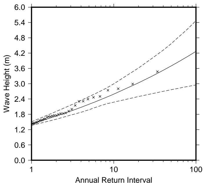
Figure 9 Extreme wave distribution for Kavala Bay. The crosses represents the wave events that occurred since 1979. The plain line is the statistical distribution that best fit the past wave events. The dotted line show the upper and lower high confidence of the fit, there is a 95% chance that the fitted distribution lie between the two dashed lines.
