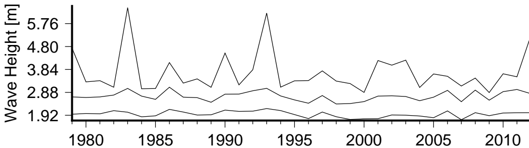
Figure 8 Annual variation in large waves (90th percentile)(lower curve), severe waves (99th percentile) (middle curve) and the largest wave(upper curve) in Hideaway Resort.
