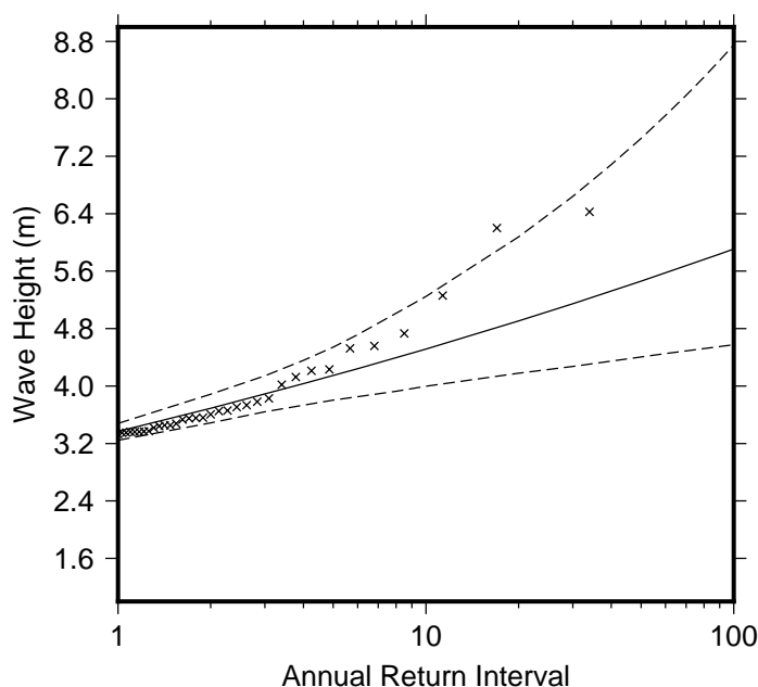
Figure 9 Extreme wave distribution for Hideaway Resort. The crosses represents the wave events that occurred since 1979. The plain line is the statistical distribution that best fit the past wave events. The dotted line show the upper and lower high confidence of the fit, there is a 95% chance that the fitted distribution lie between the two dashed lines.
