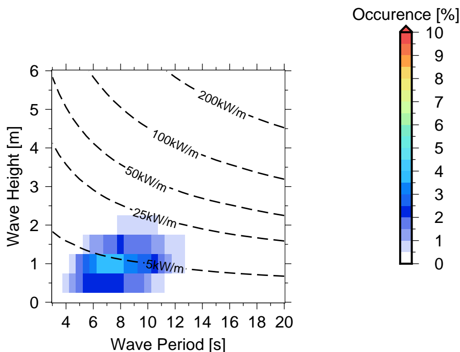
Figure 10 Occurrences of sea states in Hideaway Resort .
