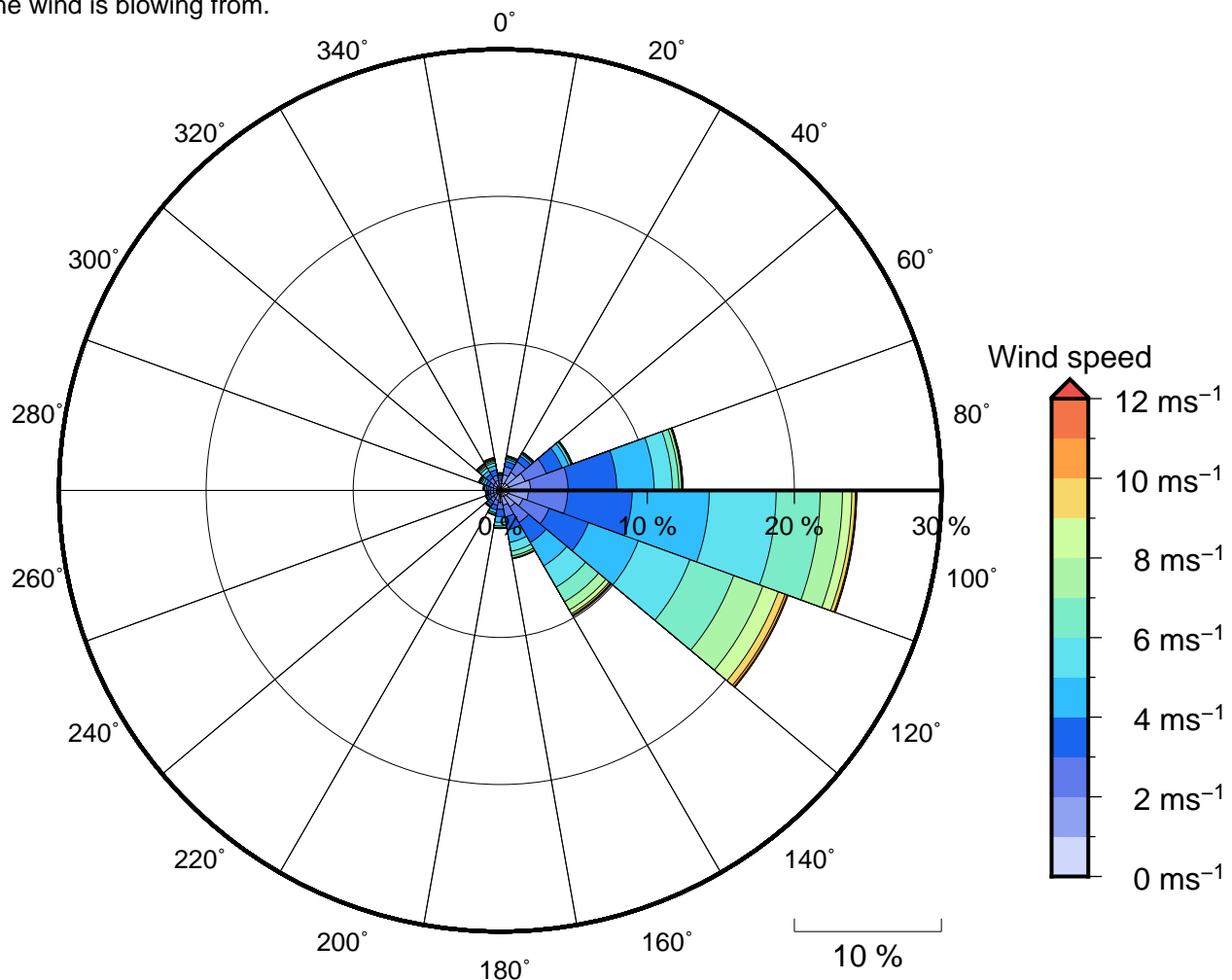
Figure 11 Annual wind rose for Hideaway Resort. Note that directions are where the wind is coming from.
