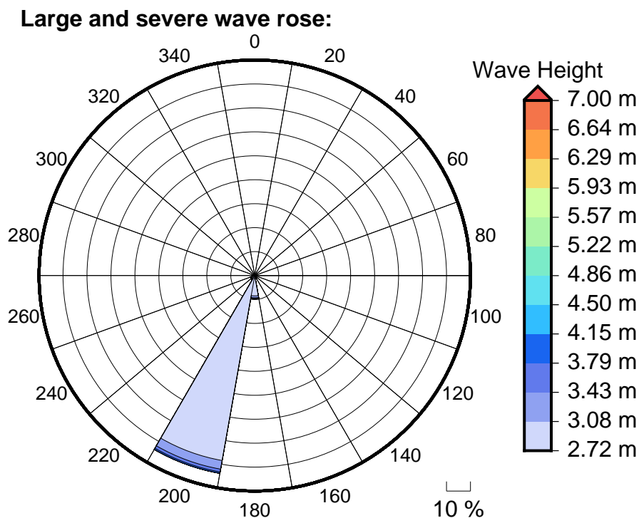
Figure 6 Large, severe and extreme wave roses for Hideaway Resort
