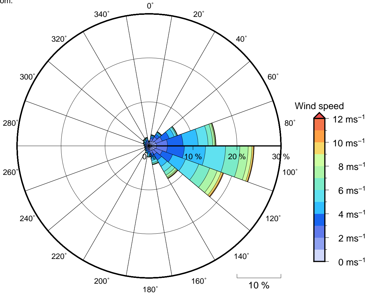
Figure 11 Annual wind rose for Galoa. Note that directions are where the wind is coming from .
