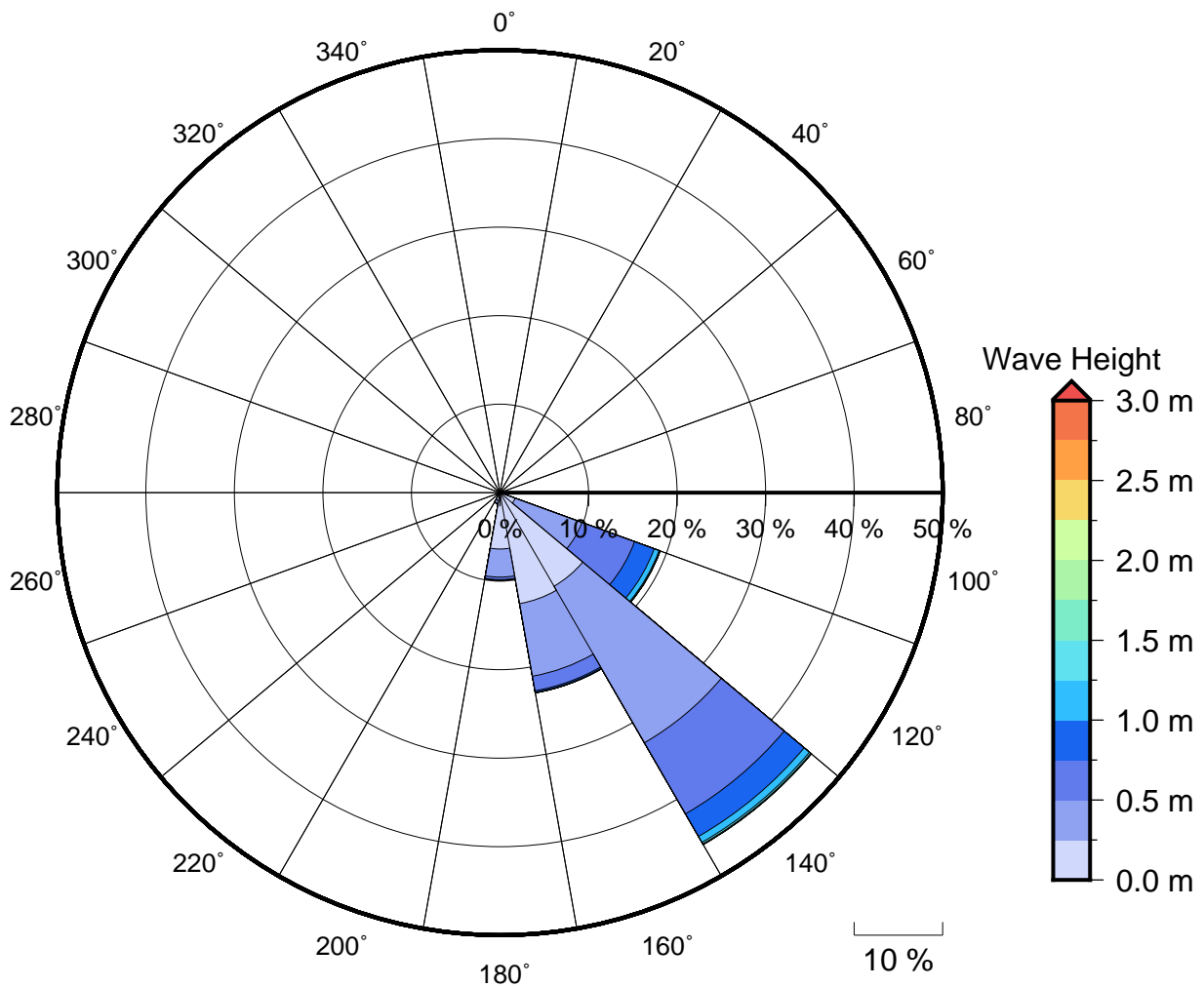
Figure 2 Annual wave rose for Galoa. Note that direction are where the wave are coming from.
