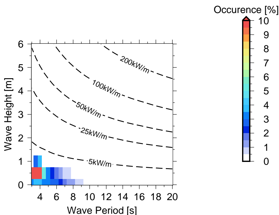
Figure 10 Occurrences of sea states in Galoa .
