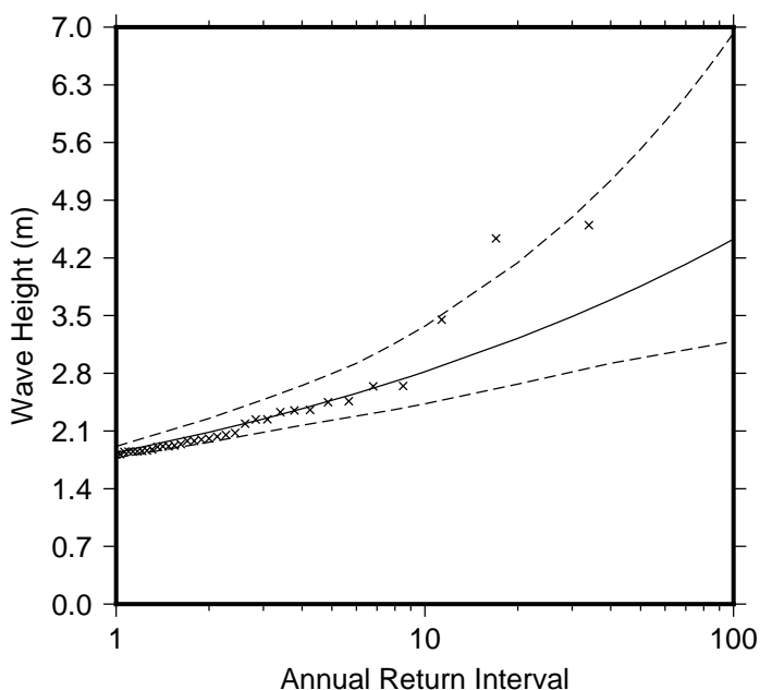
Figure 9 Extreme wave distribution for Galoa. The crosses represents the wave events that occurred since 1979. The plain line is the statistical distribution that best fit the past wave events. The dotted line show the upper and lower high confidence of the fit, there is a 95% chance that the fitted distribution lie between the two dashed lines.
