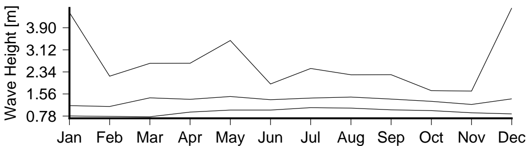
Figure 7 Monthly variation in large waves (90th percentile)(lower curve), severe waves (99th percentile) (middle curve) and the largest wave(upper curve) in Galoa.
