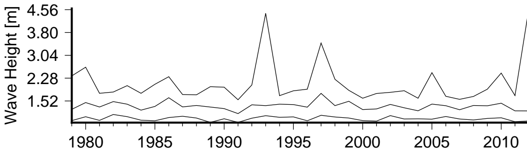
Figure 8 Annual variation in large waves (90th percentile)(lower curve), severe waves (99th percentile) (middle curve) and the largest wave(upper curve) in Galoa.
