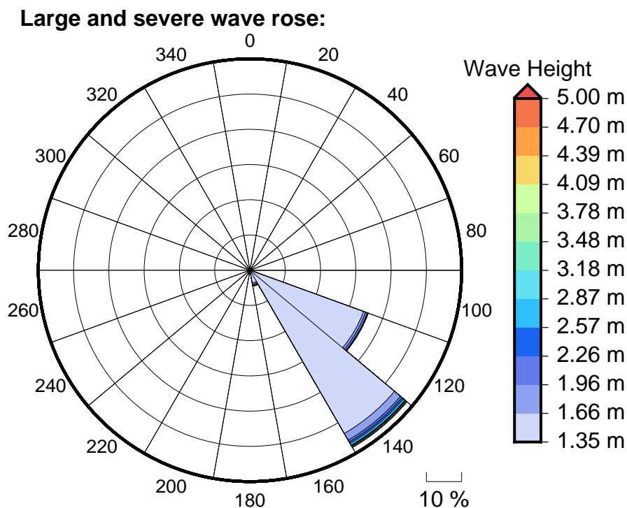
Figure 6 Large, severe and extreme wave roses for Galoa
