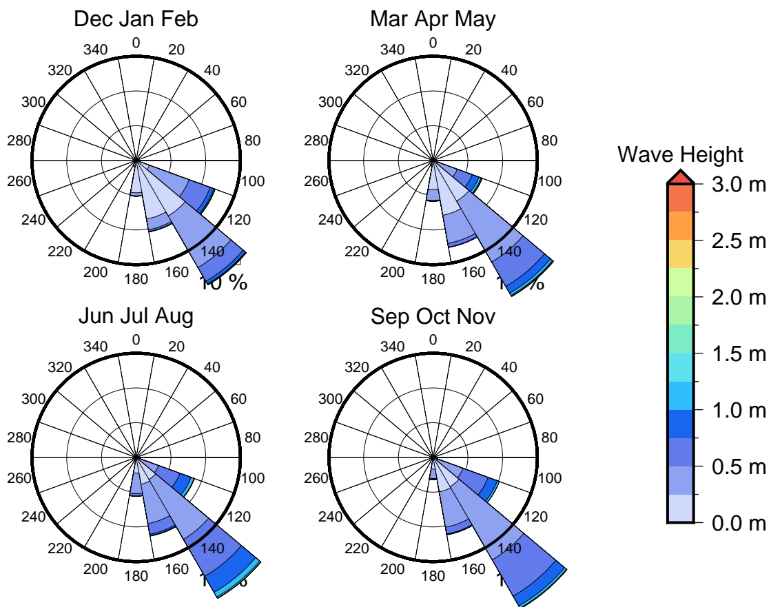
Figure 3 Seasonal wave roses for Galoa
