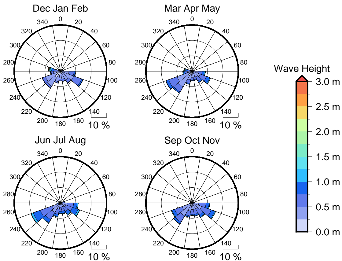
Figure 3 Seasonal wave roses for Frigates Passage
