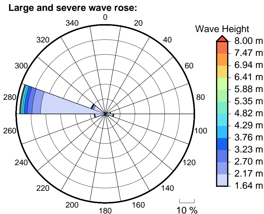
Figure 6 Large, severe and extreme wave roses for Frigates Passage
