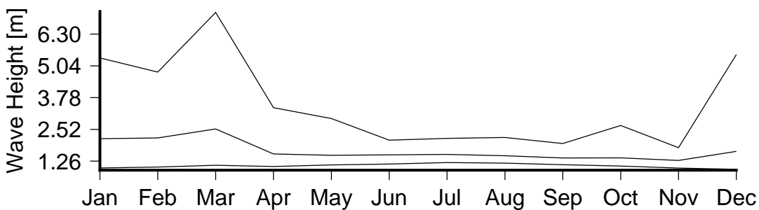
Figure 7 Monthly variation in large waves (90th percentile)(lower curve), severe waves (99th percentile) (middle curve) and the largest wave(upper curve) in Frigates Passage.
