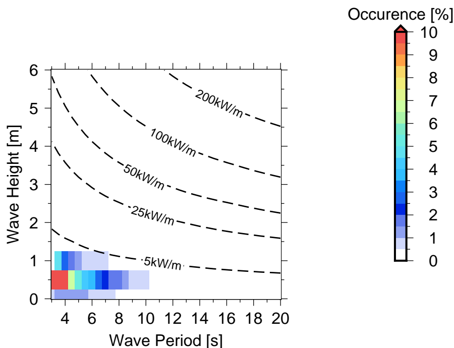
Figure 10 Occurrences of sea states in Frigates Passage .
