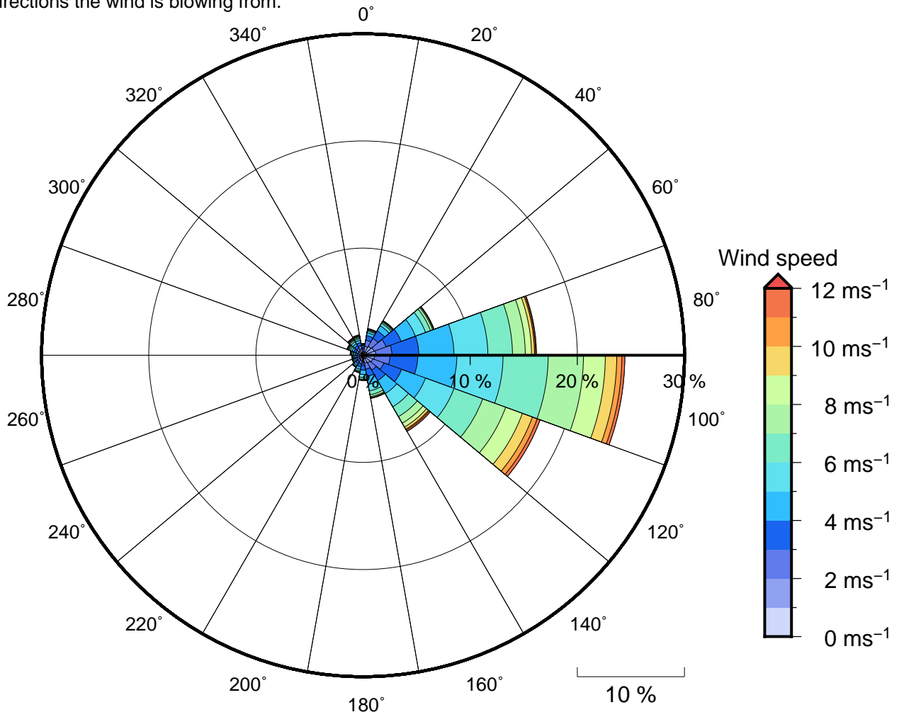
Figure 11 Annual wind rose for Frigates Passage. Note that directions are where the wind is coming from.
