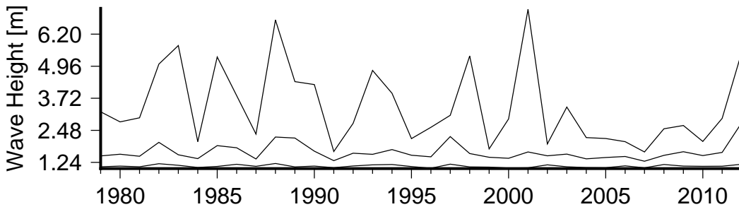
Figure 8 Annual variation in large waves (90th percentile)(lower curve), severe waves (99th percentile) (middle curve) and the largest wave(upper curve) in Frigates Passage.
