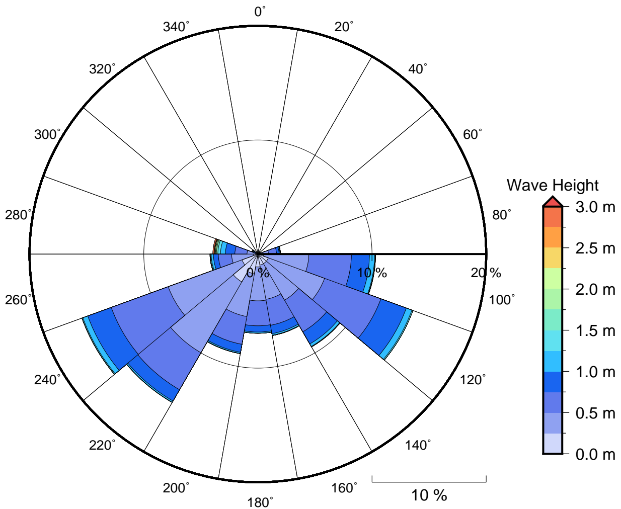
Figure 2 Annual wave rose for Frigates Passage. Note that direction are where the wave are coming from .
