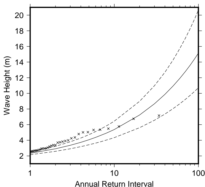
Figure 9 Extreme wave distribution for Frigates Passage. The crosses represents the wave events that occurred since 1979. The plain line is the statistical distribution that best fit the past wave events. The dotted line show the upper and lower high confidence of the fit, there is a 95% chance that the fitted distribution lie between the two dashed lines.
