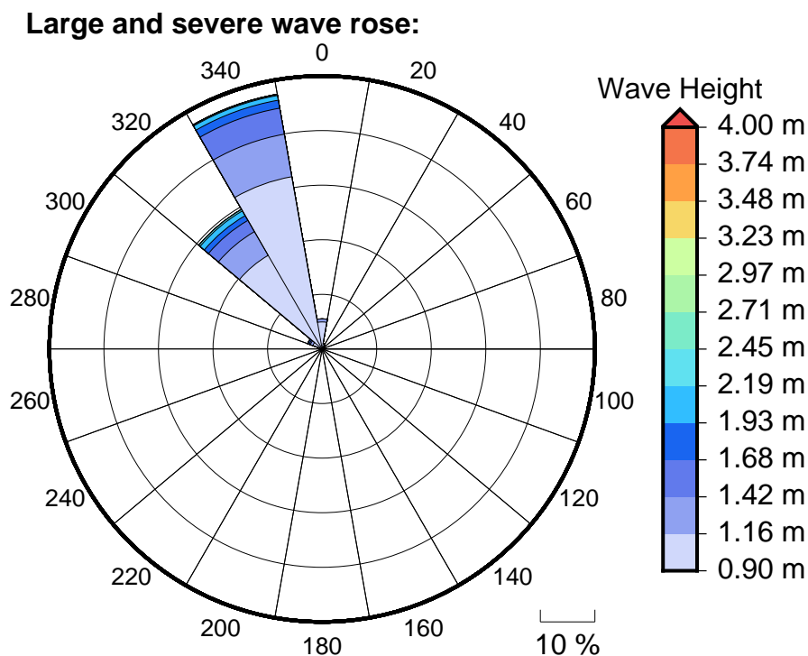
Figure 6 Large, severe and extreme wave roses for Denarau Marina
