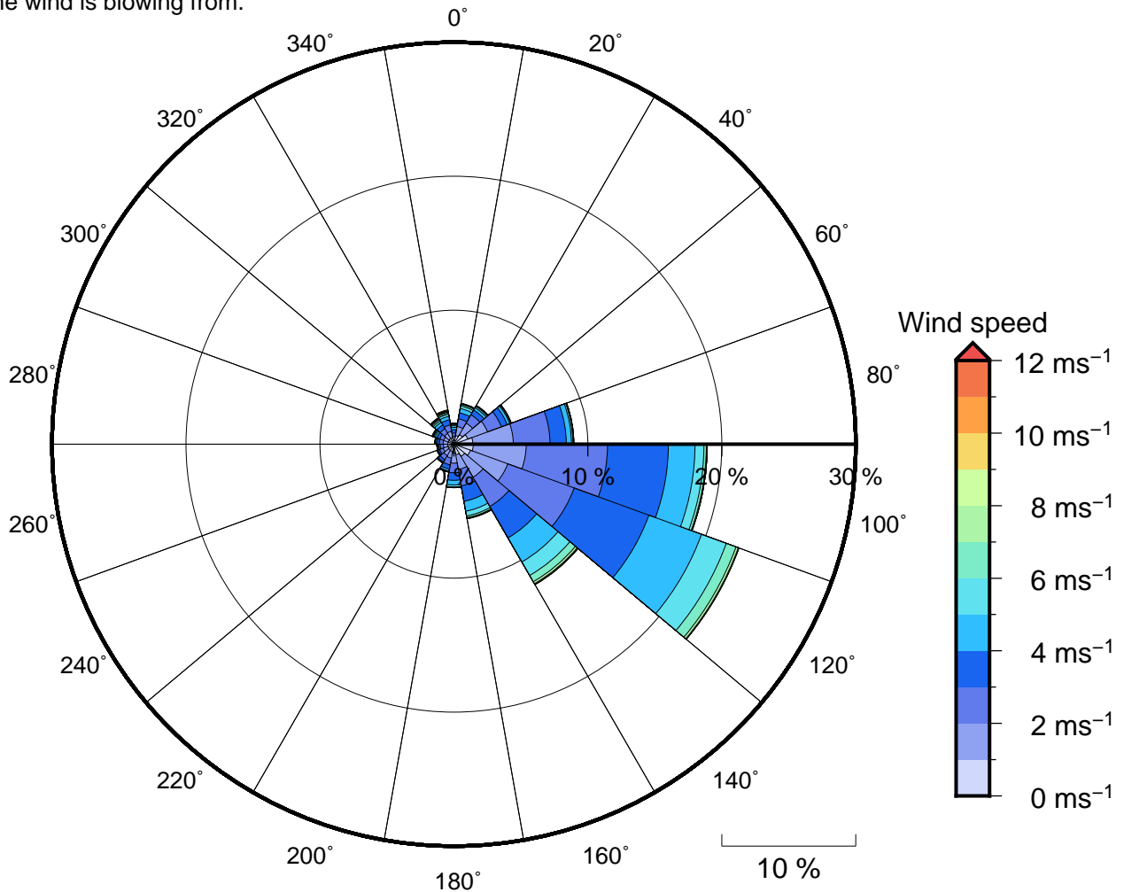
Figure 11 Annual wind rose for Denarau Marina. Note that directions are where the wind is coming from.
