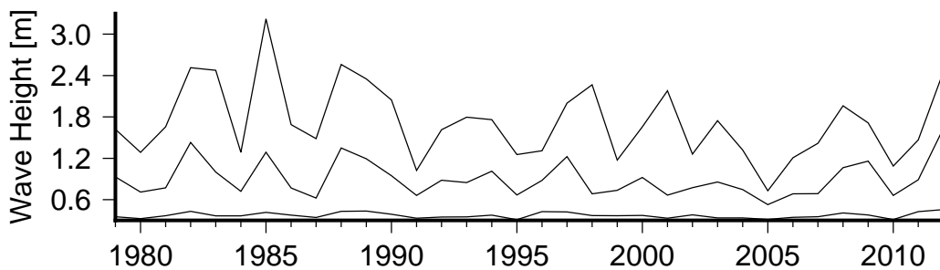
Figure 8 Annual variation in large waves (90th percentile)(lower curve), severe waves (99th percentile) (middle curve) and the largest wave(upper curve) in Denarau Marina.
