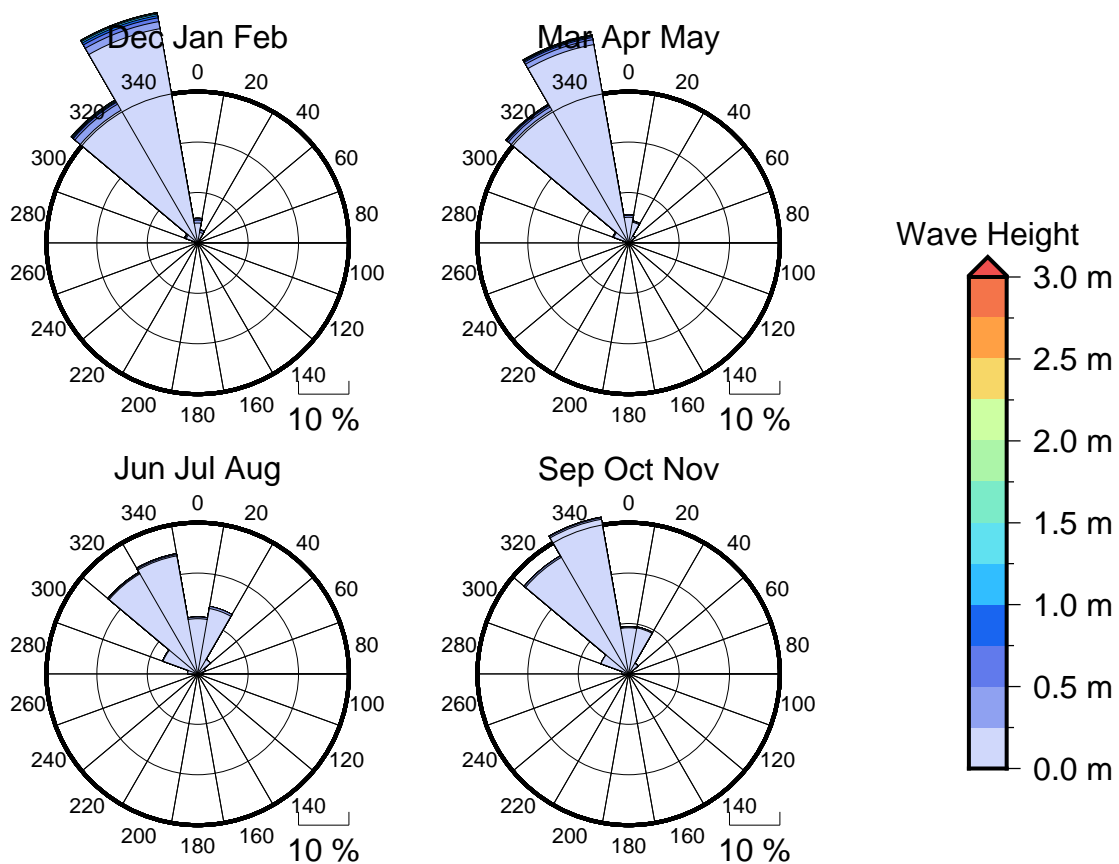
Figure 3 Seasonal wave roses for Denarau Marina
