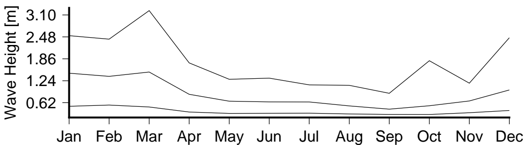
Figure 7 Monthly variation in large waves (90th percentile)(lower curve), severe waves (99th percentile) (middle curve) and the largest wave(upper curve) in Denarau Marina.
