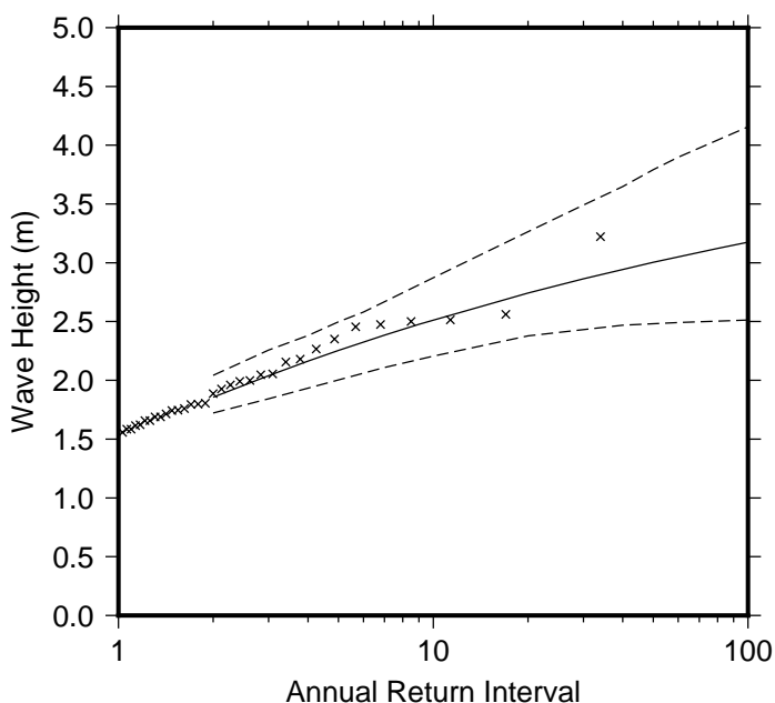
Figure 9 Extreme wave distribution for Denarau Marina. The crosses represents the wave events that occurred since 1979. The plain line is the statistical distribution that best fit the past wave events. The dotted line show the upper and lower high confidence of the fit, there is a 95% chance that the fitted distribution lie between the two dashed lines.
