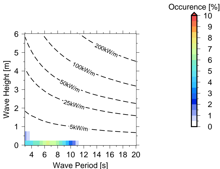
Figure 10 Occurences of sea states in Denarau Marina .
