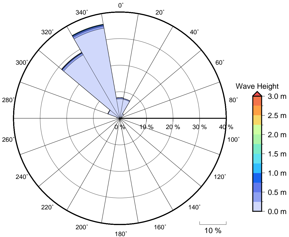
Figure 2 Annual wave rose for Denarau Marina. Note that direction are where the wave are coming from .
