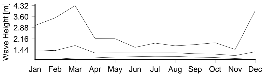
Figure 7 Monthly variation in large waves (90th percentile)(lower curve), severe waves (99th percentile) (middle curve) and the largest wave(upper curve) in Davui Island.
