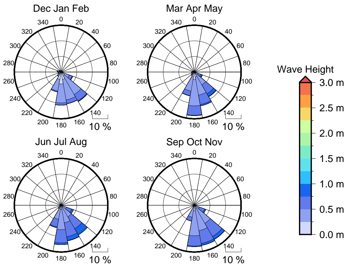
Figure 3 Seasonal wave roses for Davui Island
