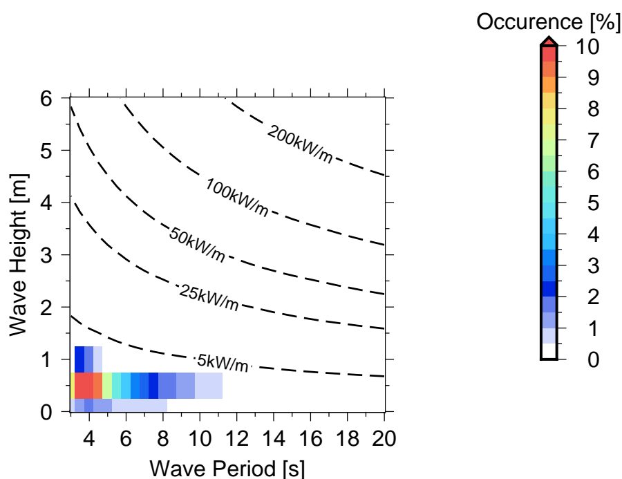
Figure 10 Occurrences of sea states in Davui Island .
