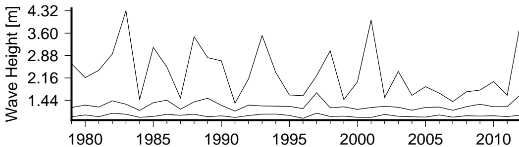
Figure 8 Annual variation in large waves (90th percentile)(lower curve), severe waves (99th percentile) (middle curve) and the largest wave(upper curve) in Davui Island.
