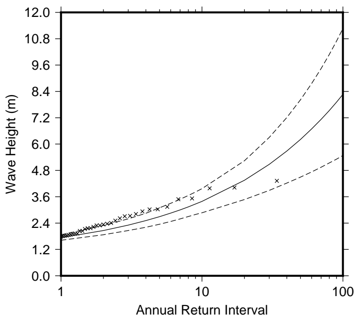
Figure 9 Extreme wave distribution for Davui Island. The crosses represents the wave events that occurred since 1979. The plain line is the statistical distribution that best fit the past wave events. The dotted line show the upper and lower high confidence of the fit, there is a 95% chance that the fitted distribution lie between the two dashed lines.
