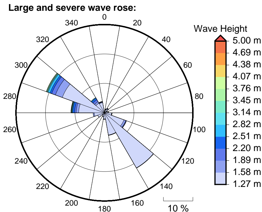
Figure 6 Large, severe and extreme wave roses for Davui Island
