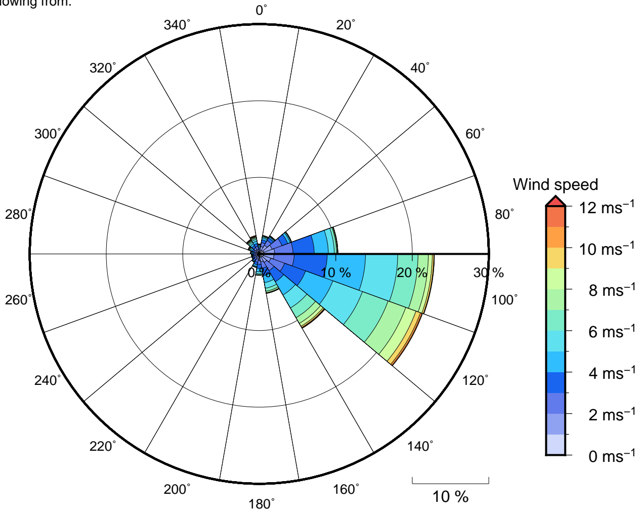
Figure 11 Annual wind rose for Cuvu Bay. Note that directions are where the wind is coming from.
