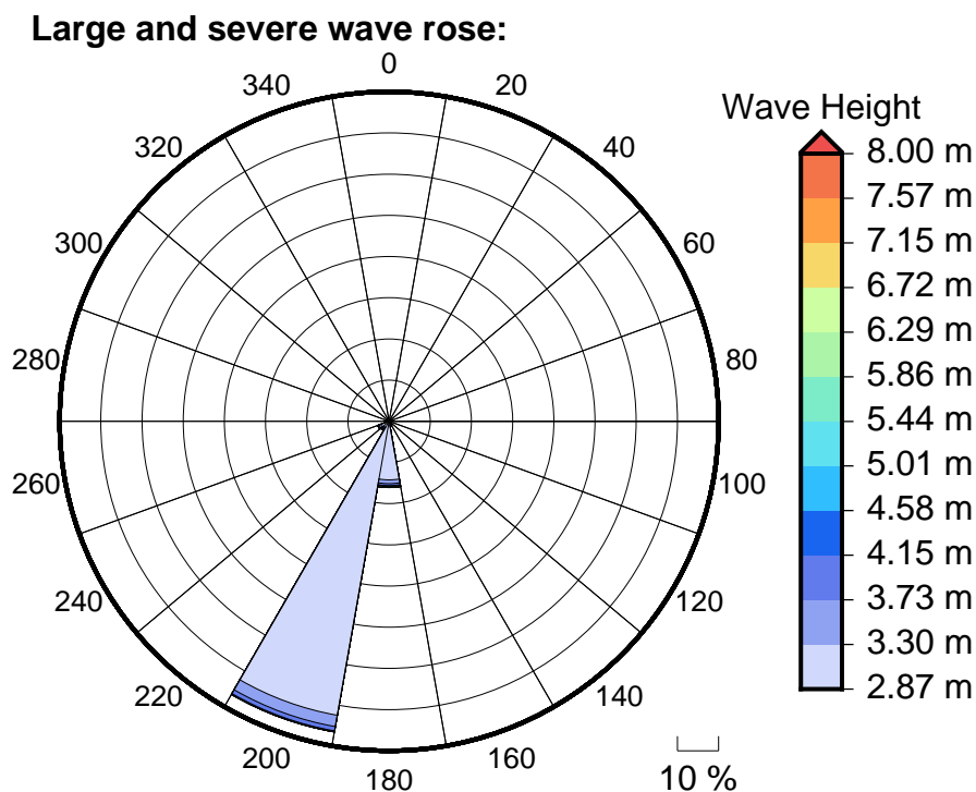
Figure 6 Large, severe and extreme wave roses for Cuvu Bay
