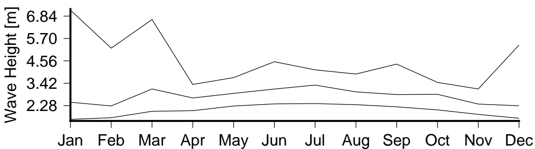
Figure 7 Monthly variation in large waves (90th percentile)(lower curve), severe waves (99th percentile) (middle curve) and the largest wave(upper curve) in Cuvu Bay.
