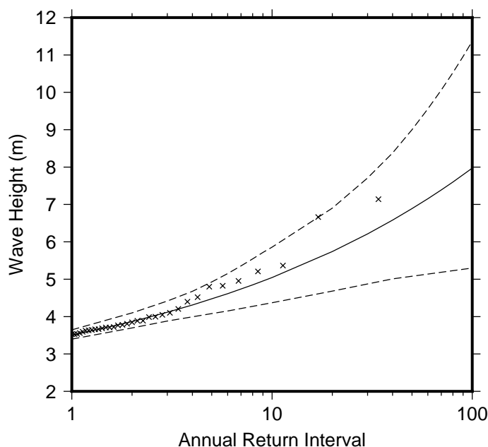
Figure 9 Extreme wave distribution for Cuvu Bay. The crosses represents the wave events that occurred since 1979. The plain line is the statistical distribution that best fit the past wave events. The dotted line show the upper and lower high confidence of the fit, there is a 95% chance that the fitted distribution lie between the two dashed lines.
