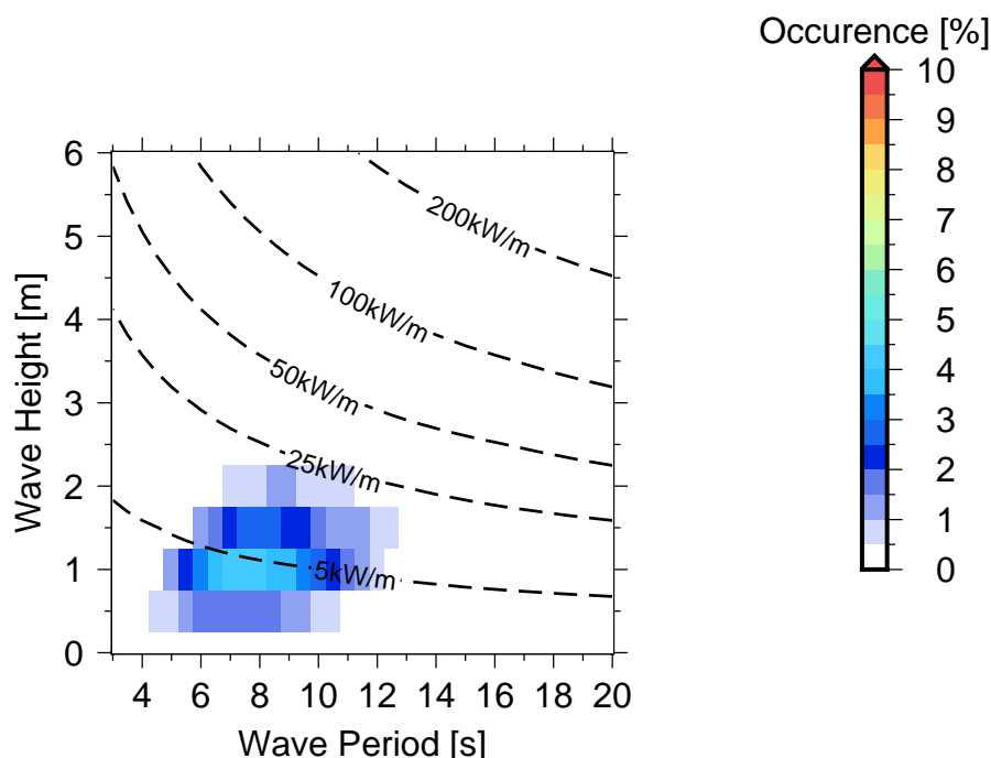
Figure 10 Occurrences of sea states in Cuvu Bay .
