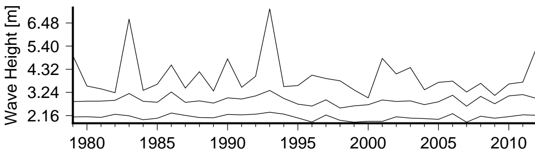
Figure 8 Annual variation in large waves (90th percentile)(lower curve), severe waves (99th percentile) (middle curve) and the largest wave(upper curve) in Cuvu Bay.
