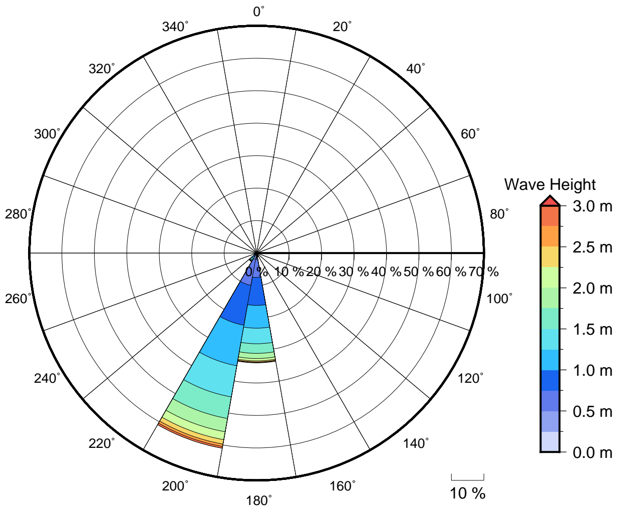
Figure 2 Annual wave rose for Cuvu Bay. Note that direction are where the wave are coming from.
