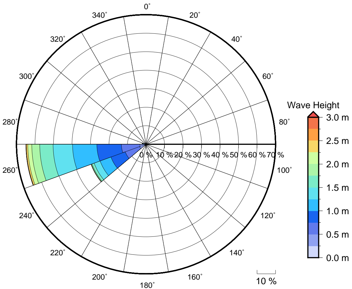
Figure 2 Annual wave rose for Cloudbreak. Note that direction are where the wave are coming from.
