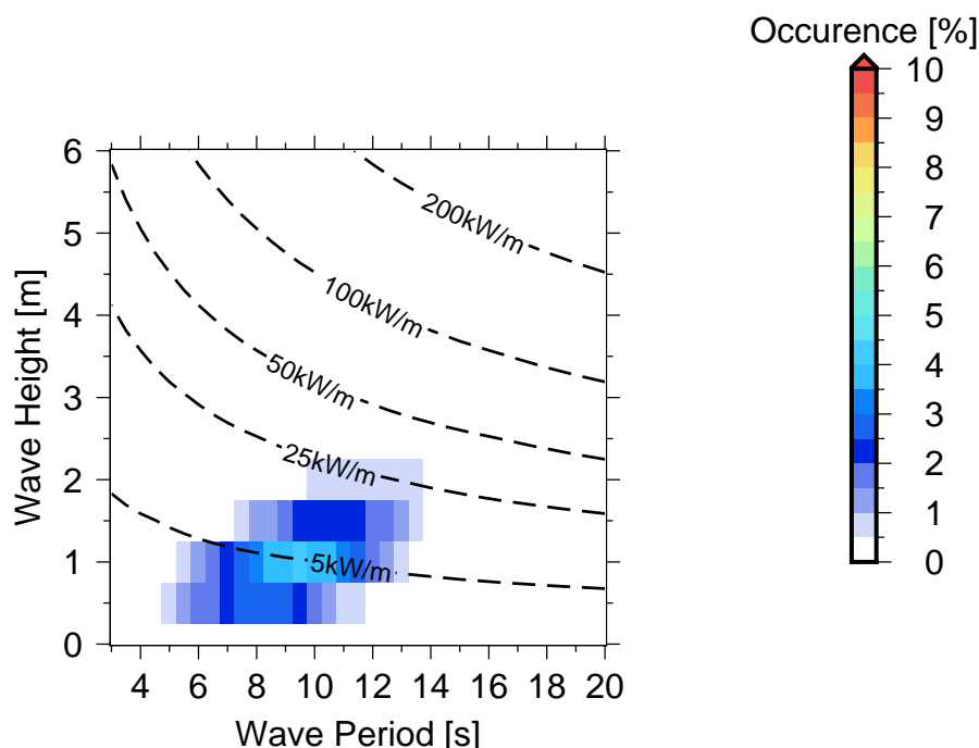
Figure 10 Occurrences of sea states in Cloudbreak .
