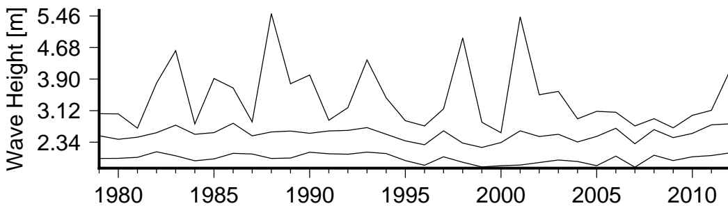
Figure 8 Annual variation in large waves (90th percentile)(lower curve), severe waves (99th percentile) (middle curve) and the largest wave(upper curve) in Cloudbreak.
