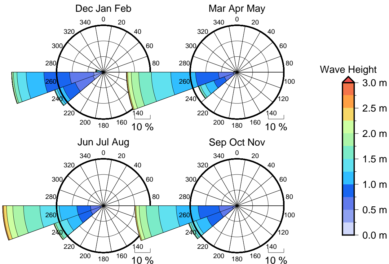
Figure 3 Seasonal wave roses for Cloudbreak
