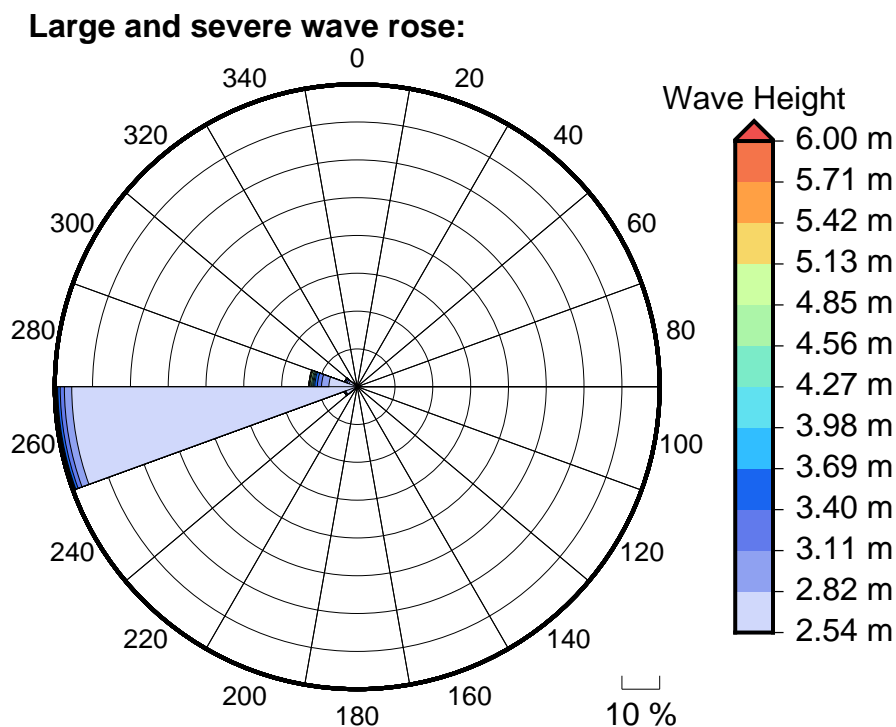
Figure 6 Large, severe and extreme wave roses for Cloudbreak
