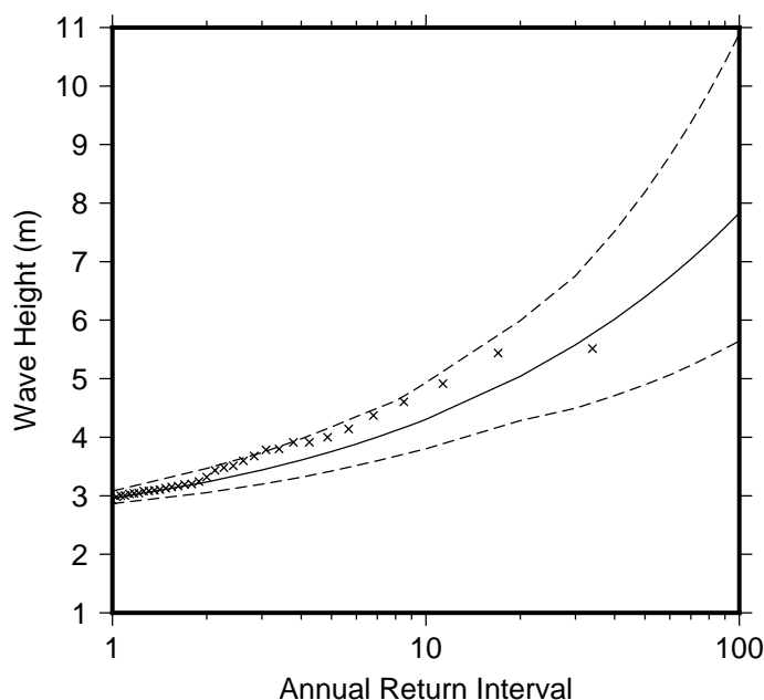
Figure 9 Extreme wave distribution for Cloudbreak. The crosses represents the wave events that occurred since 1979. The plain line is the statistical distribution that best fit the past wave events. The dotted line show the upper and lower high confidence of the fit, there is a 95% chance that the fitted distribution lie between the two dashed lines.
