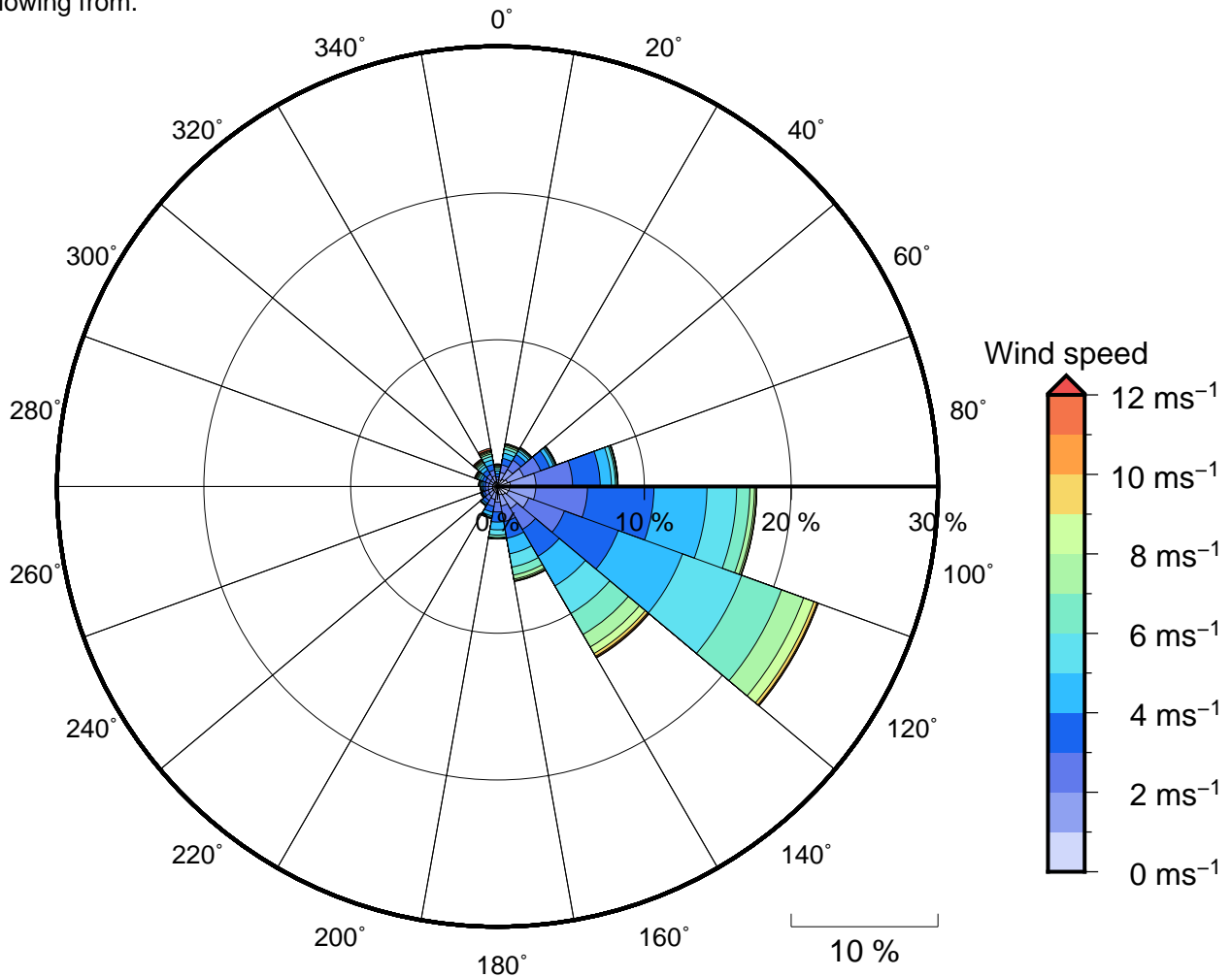
Figure 11 Annual wind rose for Cloudbreak. Note that directions are where the wind is coming from .
