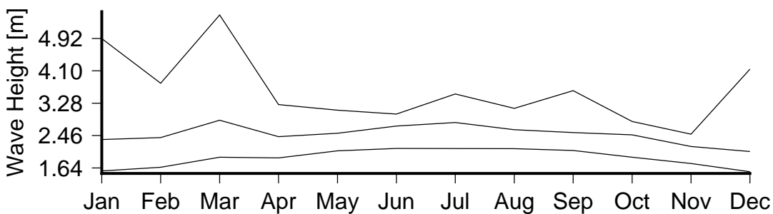
Figure 7 Monthly variation in large waves (90th percentile)(lower curve), severe waves (99th percentile) (middle curve) and the largest wave(upper curve) in Cloudbreak.
