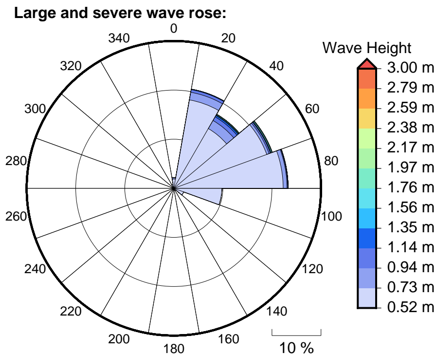
Figure 6 Large, severe and extreme wave roses for Bau
