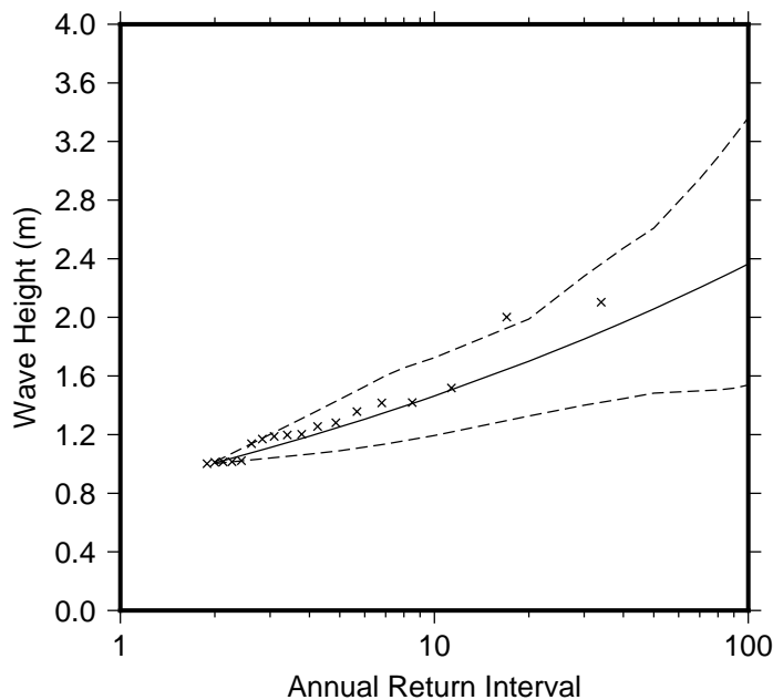
Figure 9 Extreme wave distribution for Bau. The crosses represents the wave events that occurred since 1979. The plain line is the statistical distribution that best fit the past wave events. The dotted line show the upper and lower high confidence of the fit, there is a 95% chance that the fitted distribution lie between the two dashed lines.
