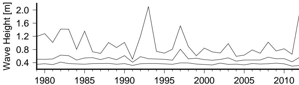
Figure 8 Annual variation in large waves (90th percentile)(lower curve), severe waves (99th percentile) (middle curve) and the largest wave(upper curve) in Bau.
