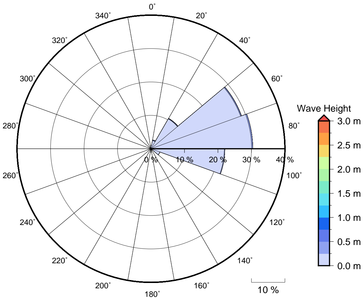
Figure 2 Annual wave rose for Bau. Note that direction are where the wave are coming from.
