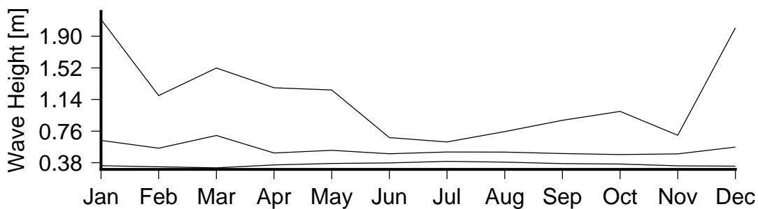
Figure 7 Monthly variation in large waves (90th percentile)(lower curve), severe waves (99th percentile) (middle curve) and the largest wave(upper curve) in Bau.
