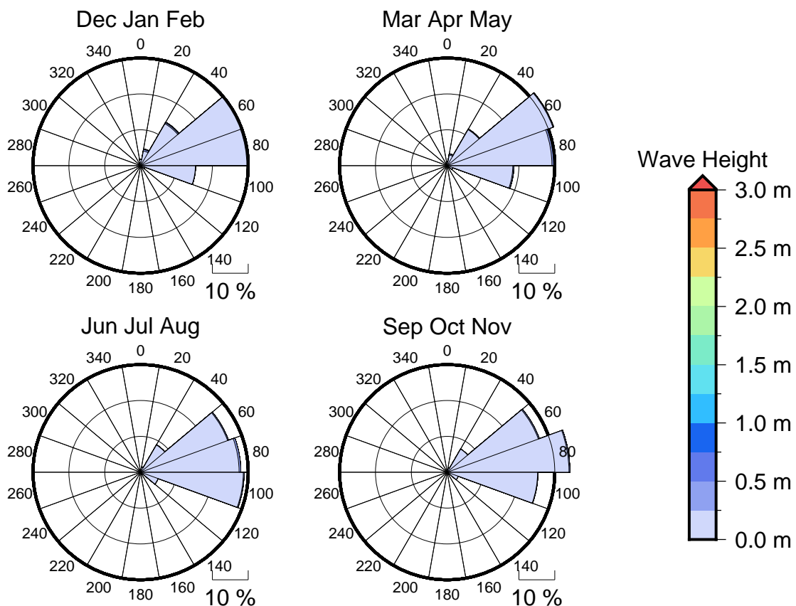
Figure 3 Seasonal wave roses for Bau
