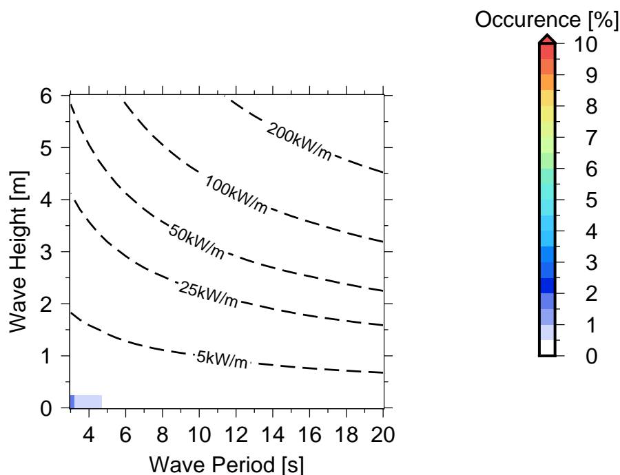
Figure 10 Occurrences of sea states in Bau .
