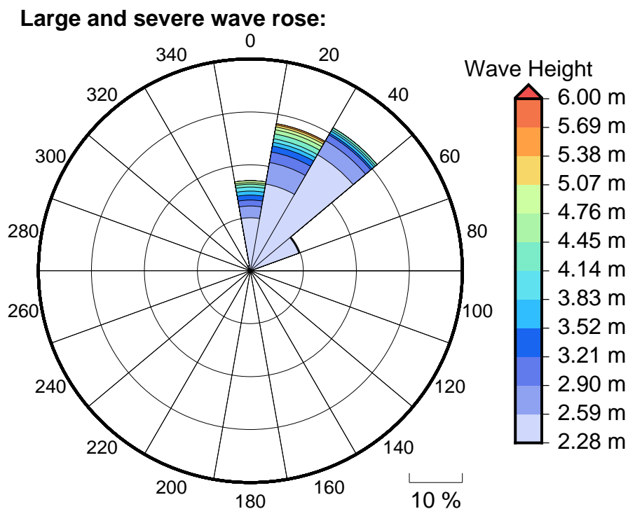
Figure 6 Large, severe and extreme wave roses for Pue
