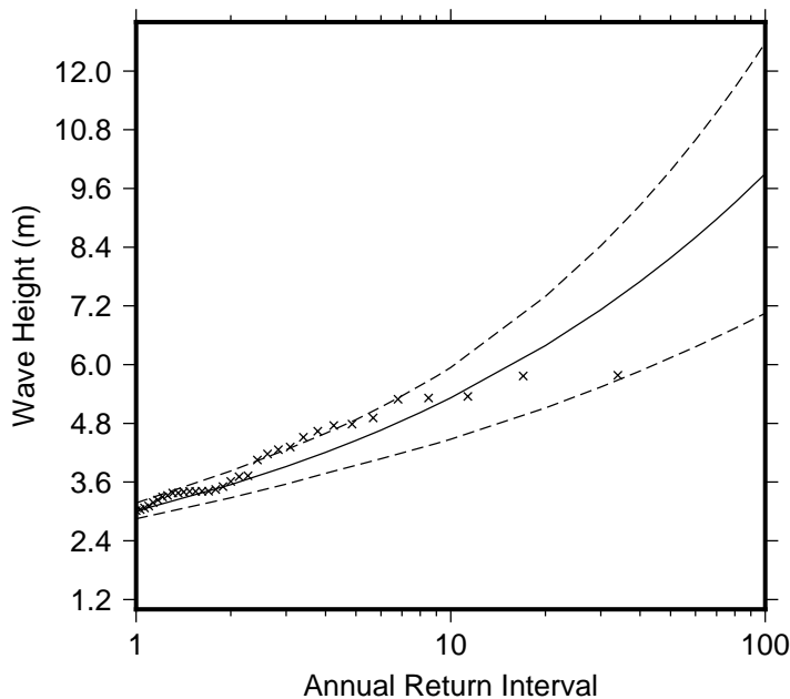
Figure 9 Extreme wave distribution for Pue. The crosses represents the wave events that occurred since 1979. The plain line is the statistical distribution that best fit the past wave events. The dotted line show the upper and lower high confidence of the fit, there is a 95% chance that the fitted distribution lie between the two dashed lines.
