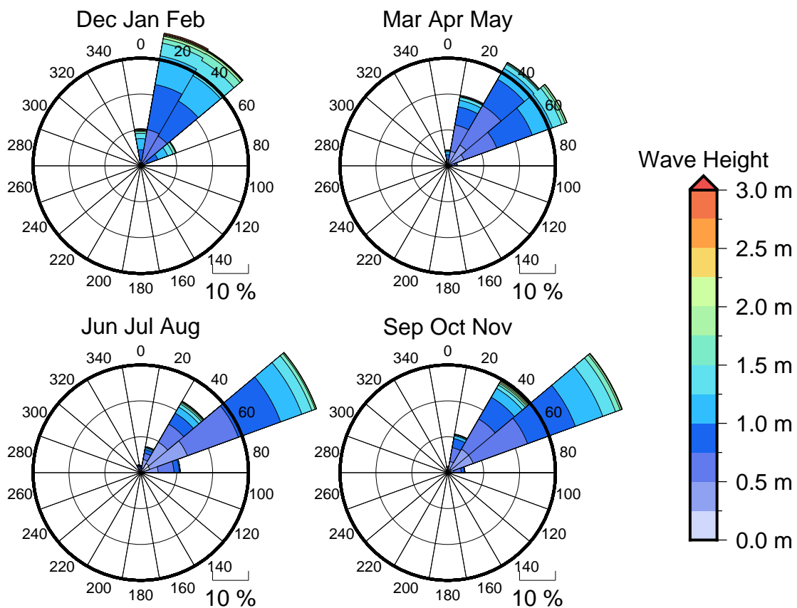
Figure 3 Seasonal wave roses for Pue
