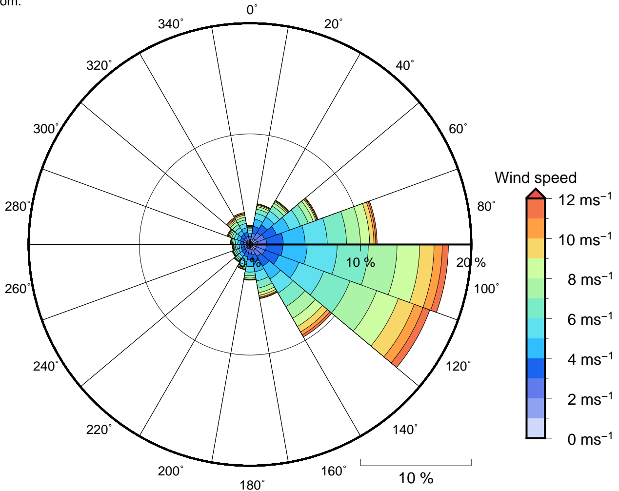
Figure 11 Annual wind rose for Pue. Note that directions are where the wind is coming from.
