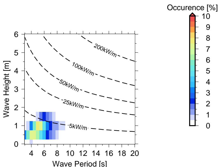
Figure 10 Occurrences of sea states in Pue .
