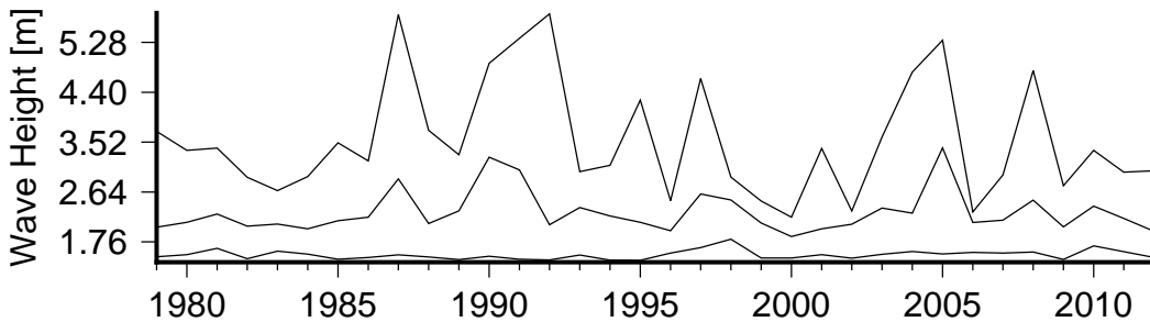
Figure 8 Annual variation in large waves (90th percentile)(lower curve), severe waves (99th percentile) (middle curve) and the largest wave(upper curve) in Pue.
