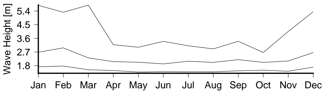
Figure 7 Monthly variation in large waves (90th percentile)(lower curve), severe waves (99th percentile) (middle curve) and the largest wave(upper curve) in Pue.
