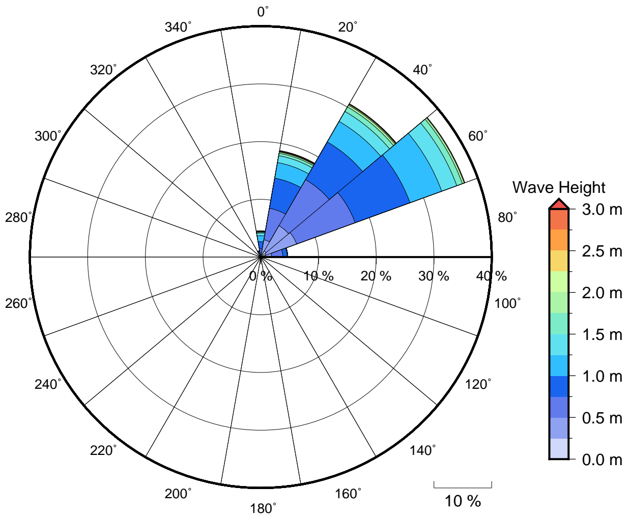
Figure 2 Annual wave rose for Pue. Note that direction are where the wave are coming from.
