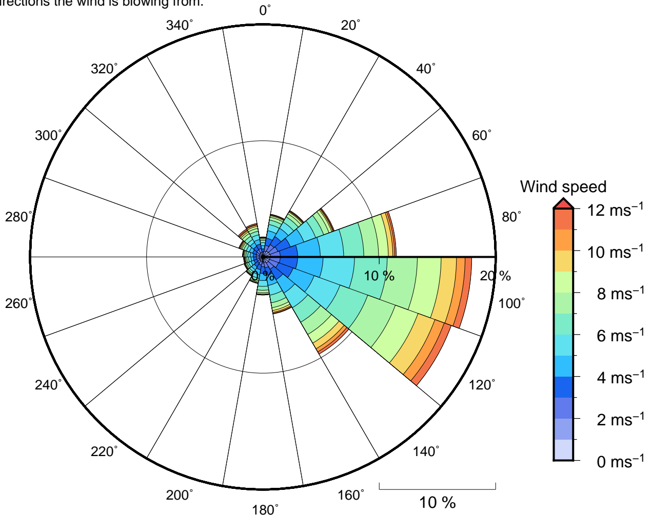
Figure 11 Annual wind rose for Papua passage. Note that directions are where the wind is coming from.
