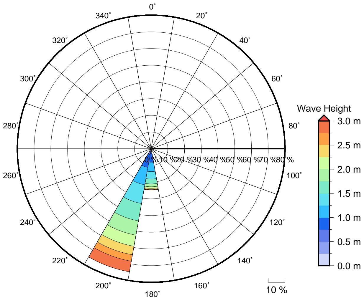
Figure 2 Annual wave rose for Papua passage. Note that direction are where the wave are coming from .
