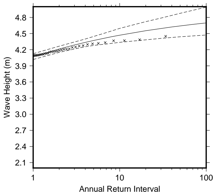
Figure 9 Extreme wave distribution for Papua passage. The crosses represents the wave events that occurred since 1979. The plain line is the statistical distribution that best fit the past wave events. The dotted line show the upper and lower high confidence of the fit, there is a 95% chance that the fitted distribution lie between the two dashed lines.
