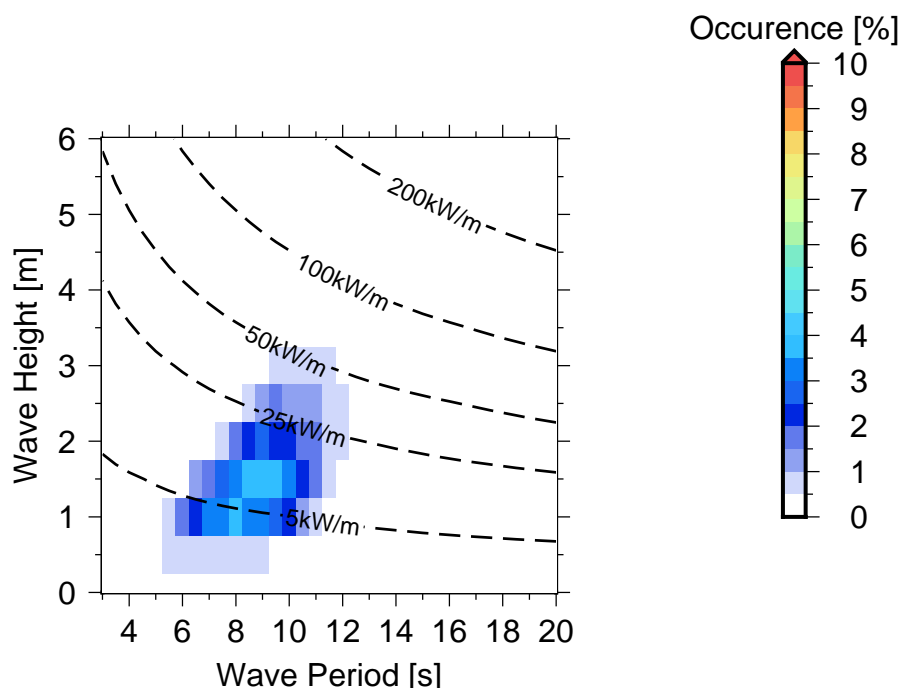
Figure 10 Occurrences of sea states in Papua passage .
